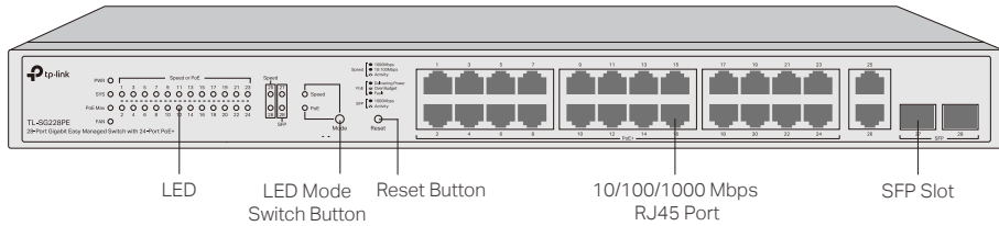
Figure 1-3 Front Panel of TL-SG228PE
