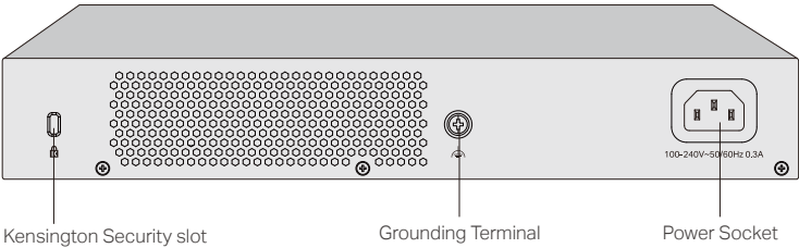
Figure 1-4 Rear Panel
