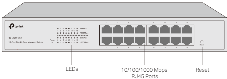
Figure 1-1 Front Panel of TL-SG216E
