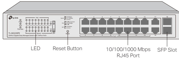
Figure 1-2 Front Panel of TL-SG220PE
