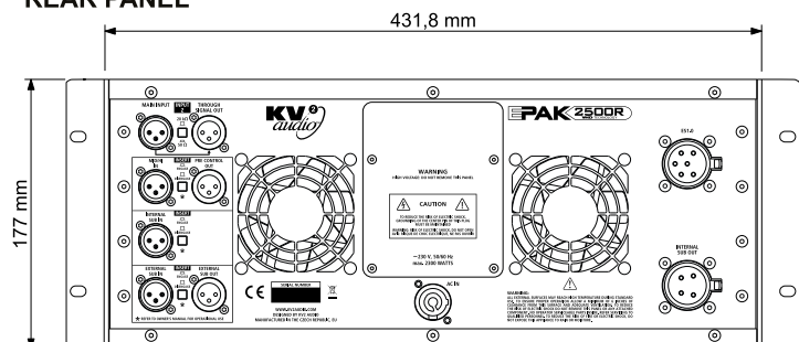
REAR PANEL
