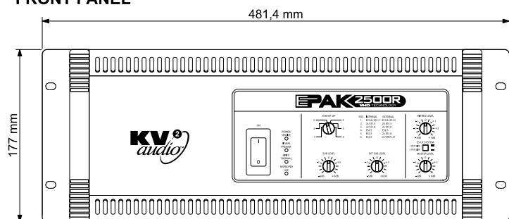
FRONT PANEL
