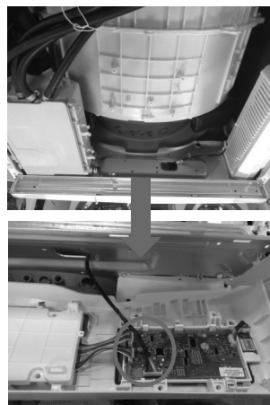
Connecting connector MAIN PWB~ Display PWB
