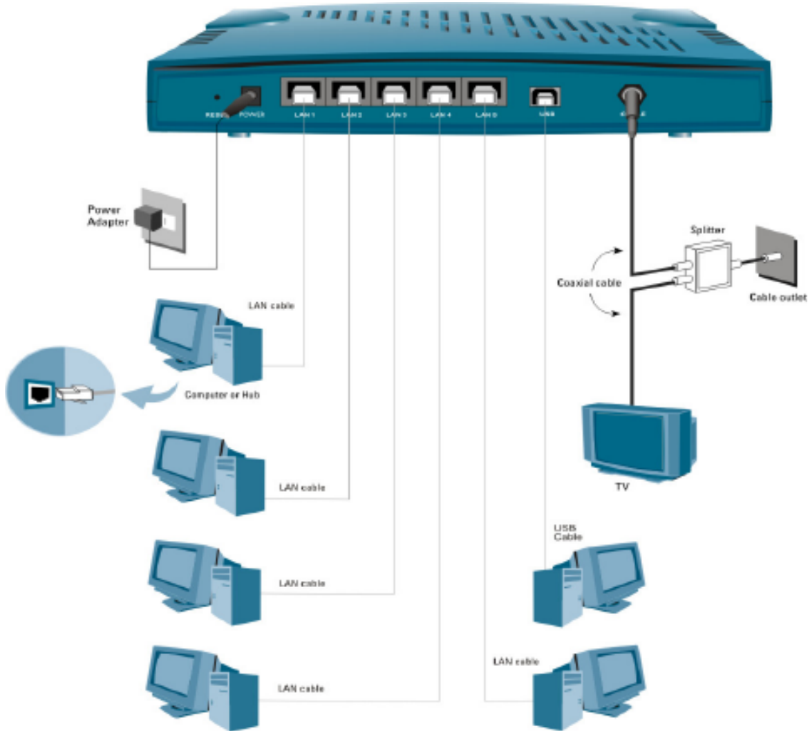
Figure 2-2 Prestige Rear Panel and Connections
