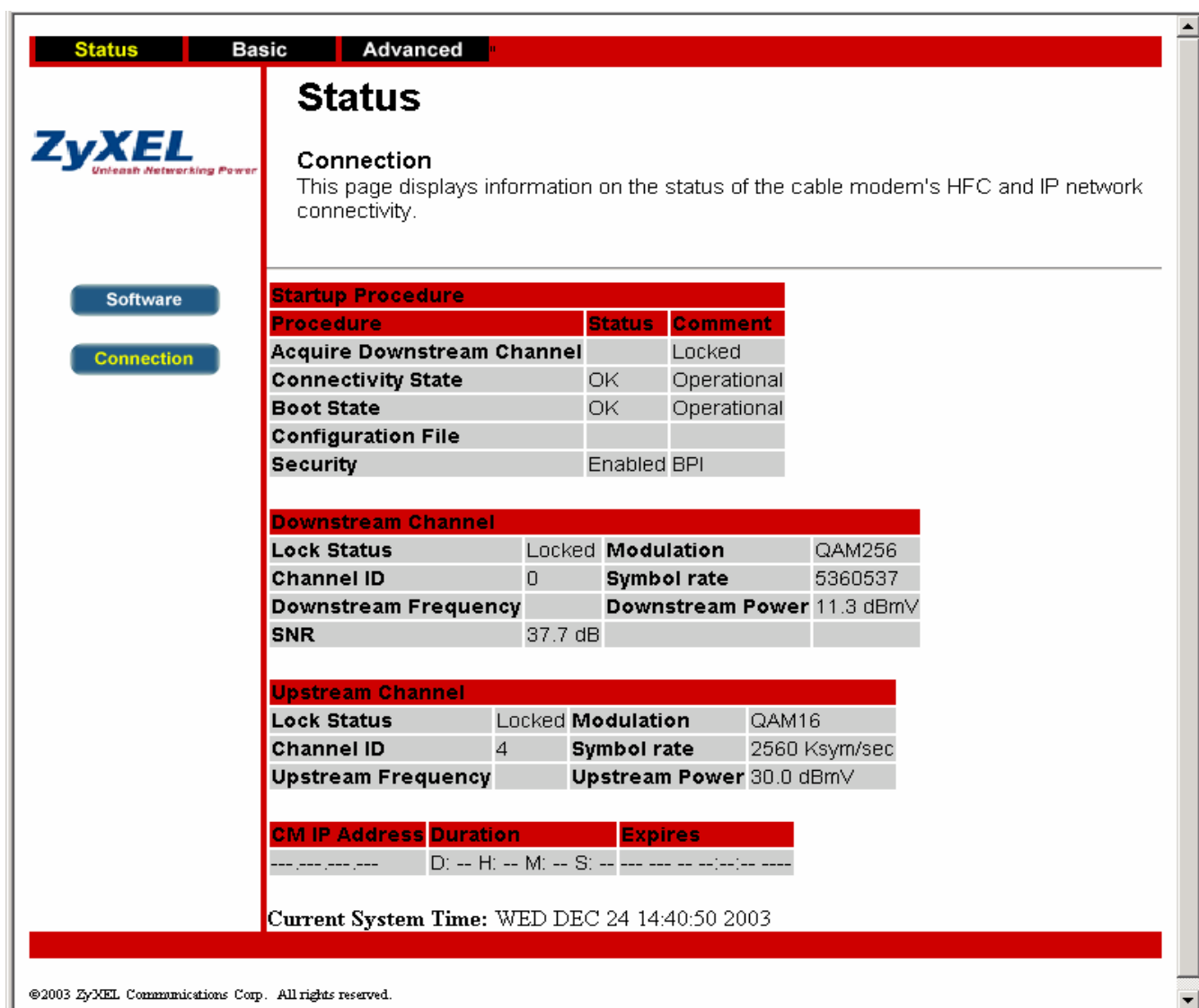
Figure 3-2 Web Management - Status
