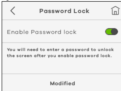
Figure 40 Password Lock
