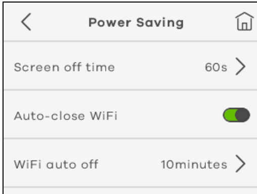
Figure 8 Power Saving
