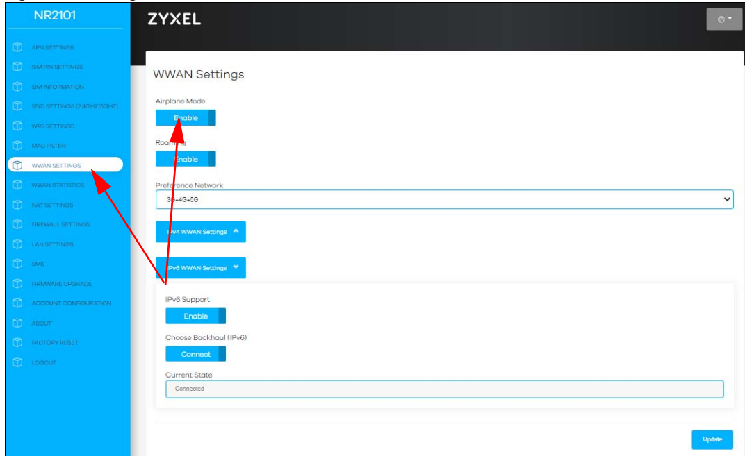
Figure 52 Navigation Panel
