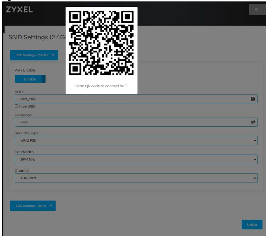
Figure 68 SSID SETTINGS-2.4 GHz &gt; SSID
