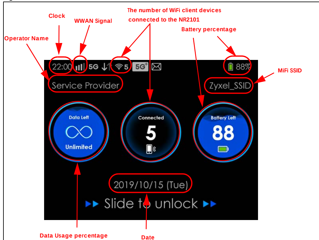
Figure 2 Home Screen
