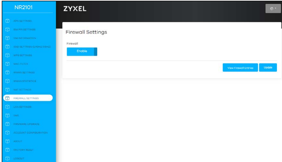
Figure 91 FIREWALL SETTINGS
