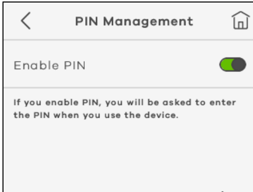
Figure 37 PIN Management
