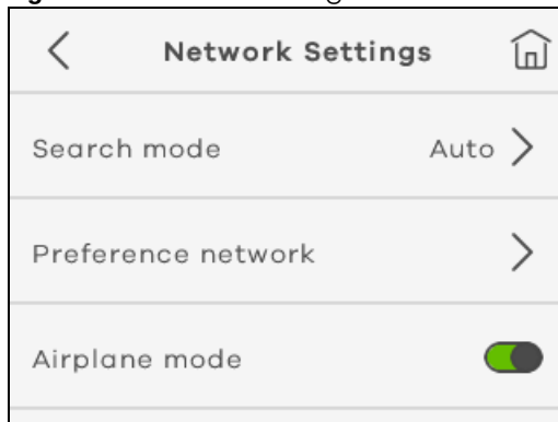
Figure 36 Network Settings
