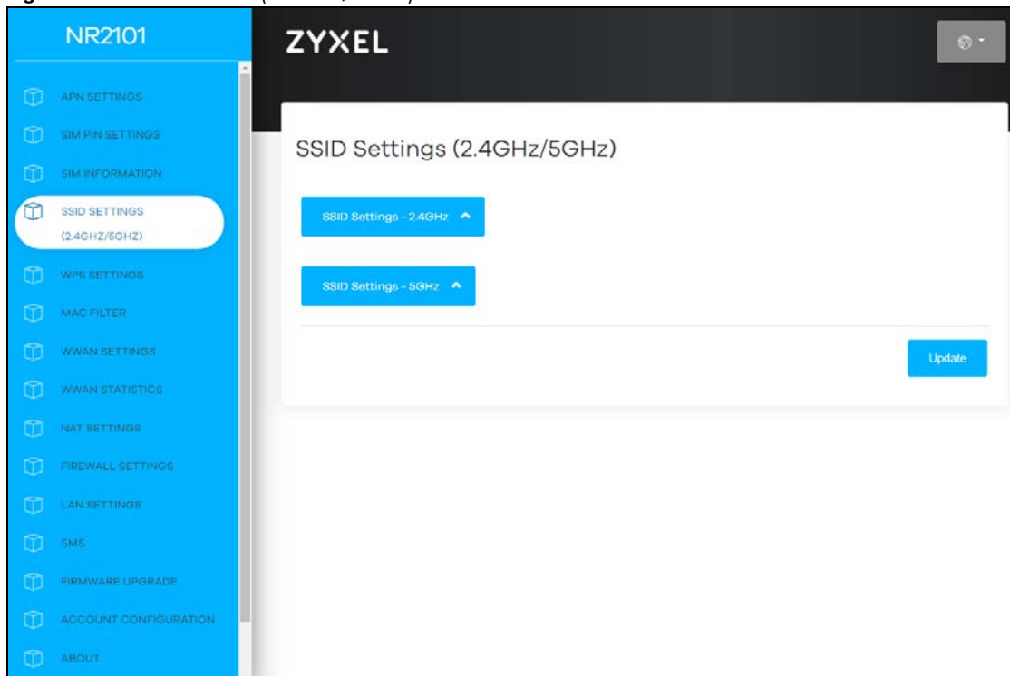
Figure 65 SSID SETTINGS(2.4GHZ/5GHZ)
