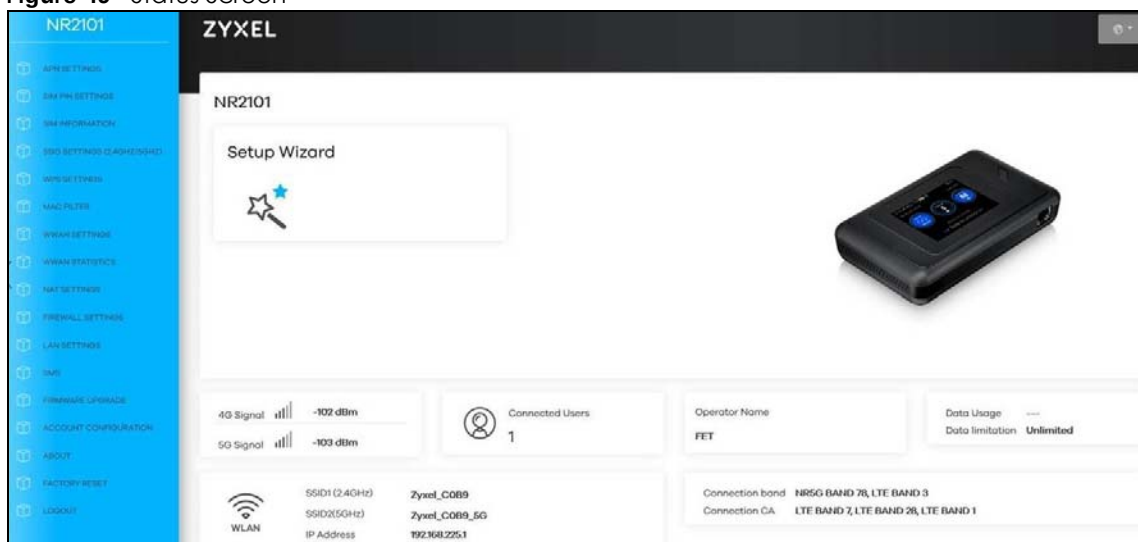
Figure 50 Screen Layout
