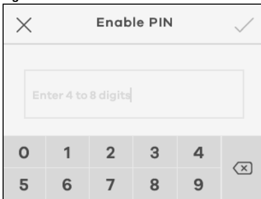
Figure 38 Enable PIN
