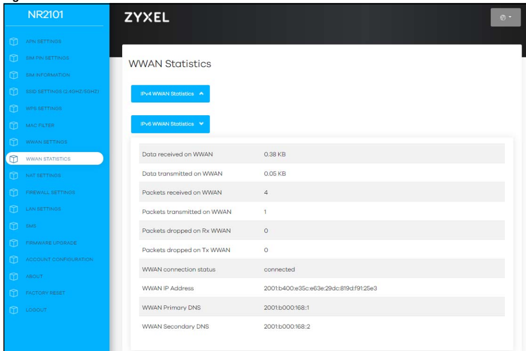
Figure 85 IPv6WWAN Statistics
