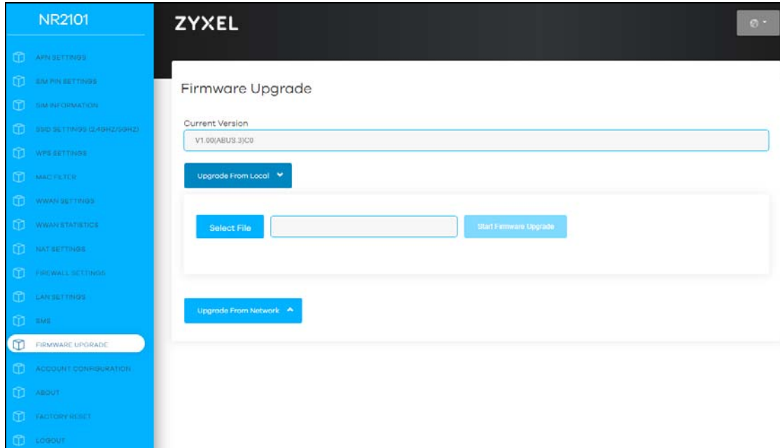
Figure 98 Firmware Upgrade
