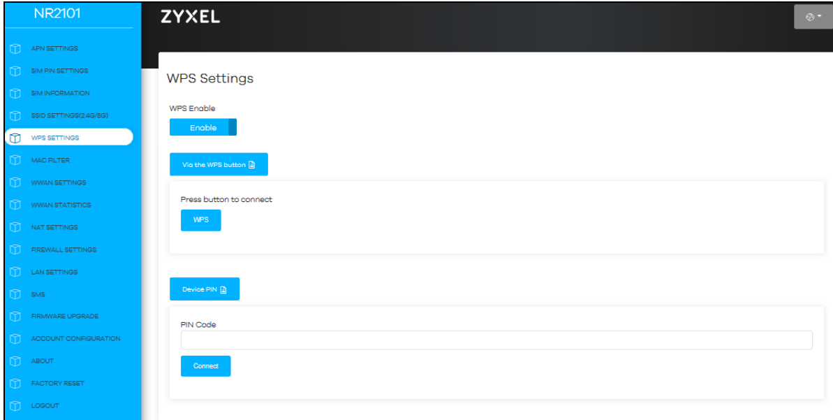
Figure 78 WPS SETTINGS
