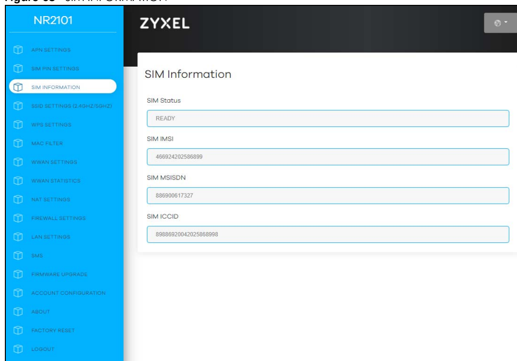
Figure 63 SIM INFORMATION
