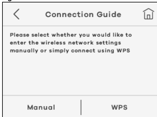
Figure 6 Connection Guide
