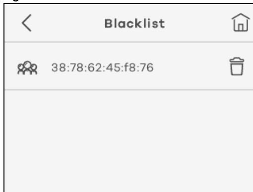
Figure 24 Blacklist
