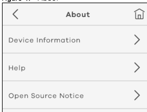
Figure 47 About
