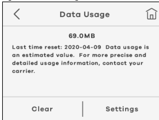
Figure 27 Data Usage
