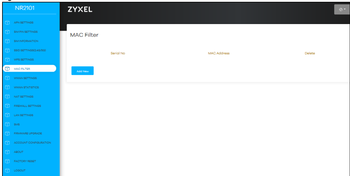
Figure 79 MAC FILTER
