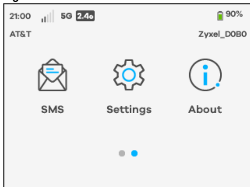
Figure 5 Menu Screen
