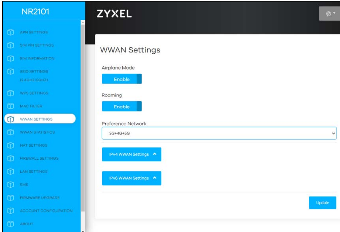
Figure 80 WWAN SETTINGS
