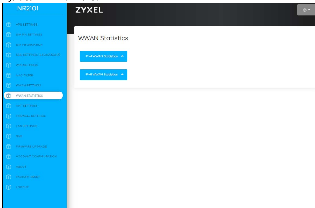
Figure 83 WWAN STATISTICS
