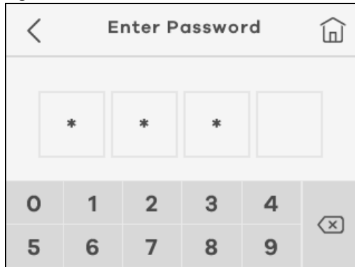
Figure 41 Enter Password
