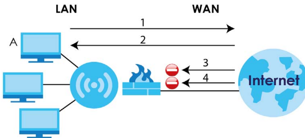
Figure 90 Default Firewall Action
