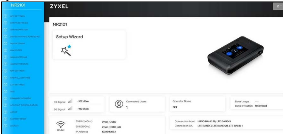
Figure 59 Status
