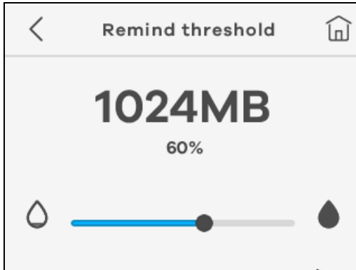
Figure 30 Remind Threshold
