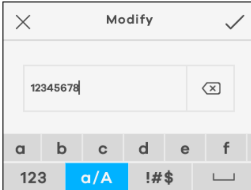
Figure 13 Modify
