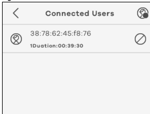
Figure 23 Connected Users
