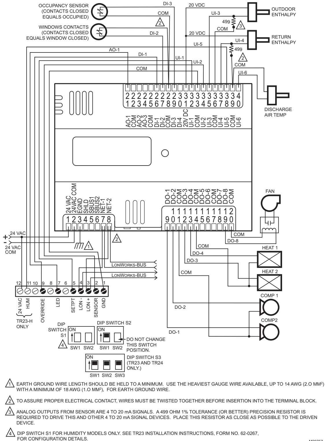
Fig. 22. Controller wiring diagram (model CP-UL6438S shown) with 4 to 20 mA enthalpy sensors and digital inputs. (For note 2, refer to Fig. 15.)
