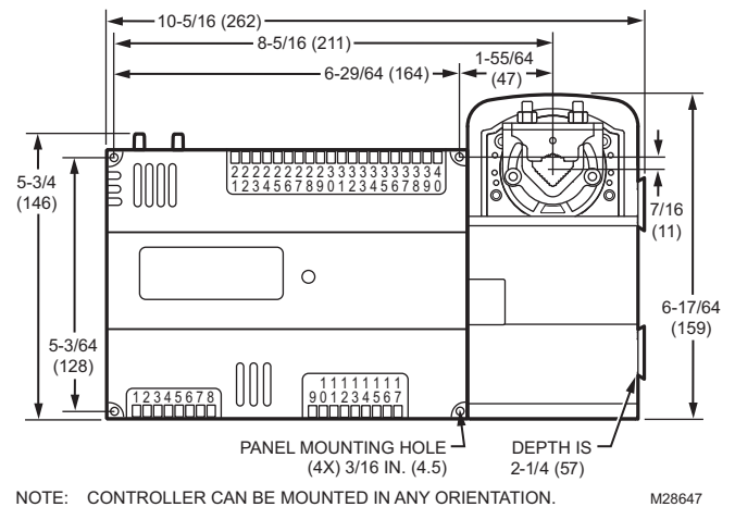
Fig. 5. Panel mounting — controller and actuator dimensions in inches (mm) for CP-VL6436AS only.
