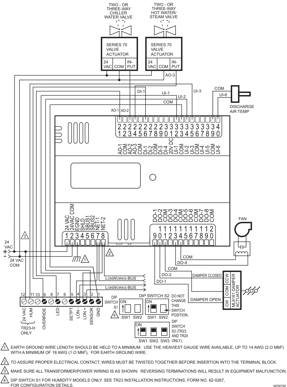
Fig. 23. Controller wiring diagram (model CP-UL6438S shown) with 4 to 20 mA heating, cooling, and model ML6161 damper actuator. (For note 2, refer to Fig. 15.)
