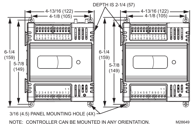
Fig. 6. Panel mounting — controller dimensions in inches (mm) for CP-UL1012S, CP-UL4024S, and CP-VL4024NS only (CP-UL4024S and CP-VL4024NS shown).
