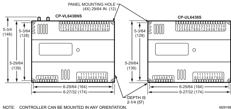
Fig. 7. Panel mounting — controller dimensions in inches (mm) for models CP-UL6438S and CP-VL6438NS only.
