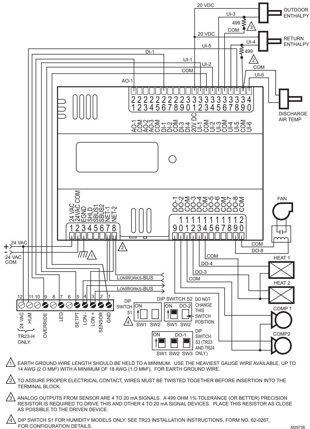
Fig. 21. Controller wiring diagram (model CP-UL6438S shown) for typical AHU application. (For note 2, refer to Fig. 15.)
