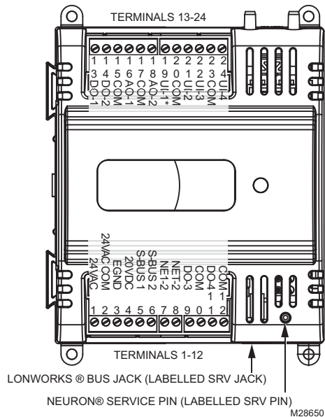
Fig. 17. Controller terminal connections, NEURON® Service Pin and LONWORKS® Bus Jack for the CP-UL1012S, CP-UL4024S, CP-VL0000AS, CP-VL4022AS, and CP-VL4024NS (CP-VL4024NS shown).
