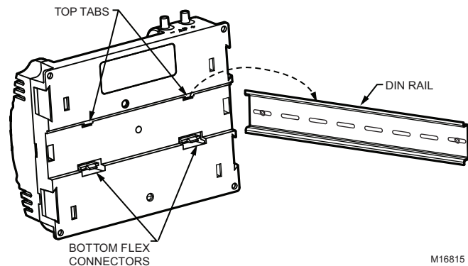
Fig. 8. Controller DIN rail mounting (models CP-UL1012S, CP-UL4024S, CP-UL6438S, CP-VL4024NS, and CP-VL6438NS).
