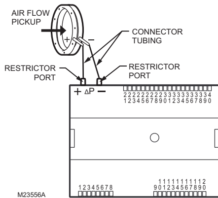
Fig. 9. Air flow pickup connections (CP-VL0000AS, CP-VL4022AS, CP-VL4024NS, CP-VL6436AS, and CP-VL6438NS).
