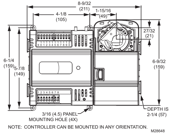
Fig. 4. Panel mounting — controller and actuator dimensions in inches (mm) for CP-VL0000AS and CP-VL4022AS only (CP-VL4022AS shown).
