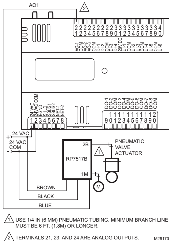
Fig. 24. Controller wiring diagram (model CP-UL6438S shown) for RP7517B pneumatic transducer.
