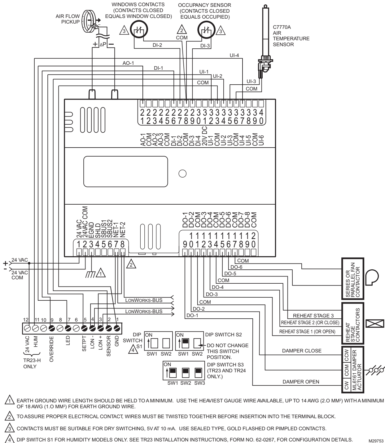
Fig. 18. Controller wiring diagram (model CP-VL6438NS shown) for typical VAV application, using the TR23 wall module and a C7770A air temperature sensor. (For note 2, refer to Fig. 15.)
