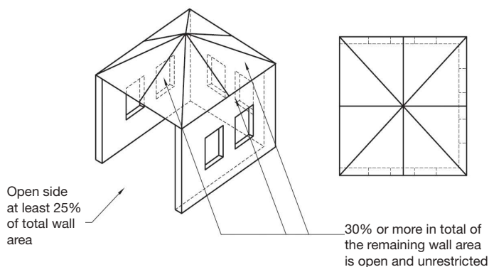
Figure 1e - Outdoor Area Example 5 Partial enclosure with overhead cover, more than two walls
