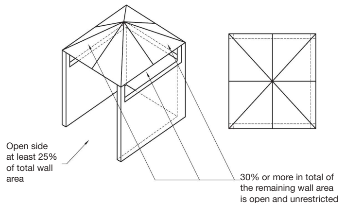
Figure 1d - Outdoor Area Example 4 Partial enclosure with overhead cover, more than two walls
