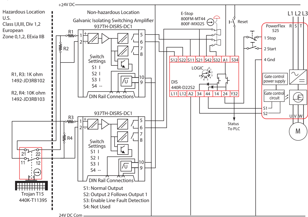
Figure 29 - Hazardous Location
