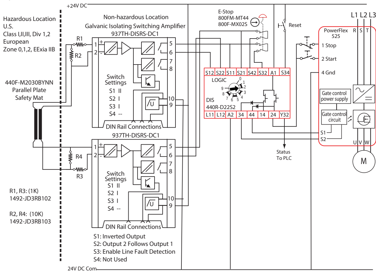
Figure 30 - Hazardous Location
