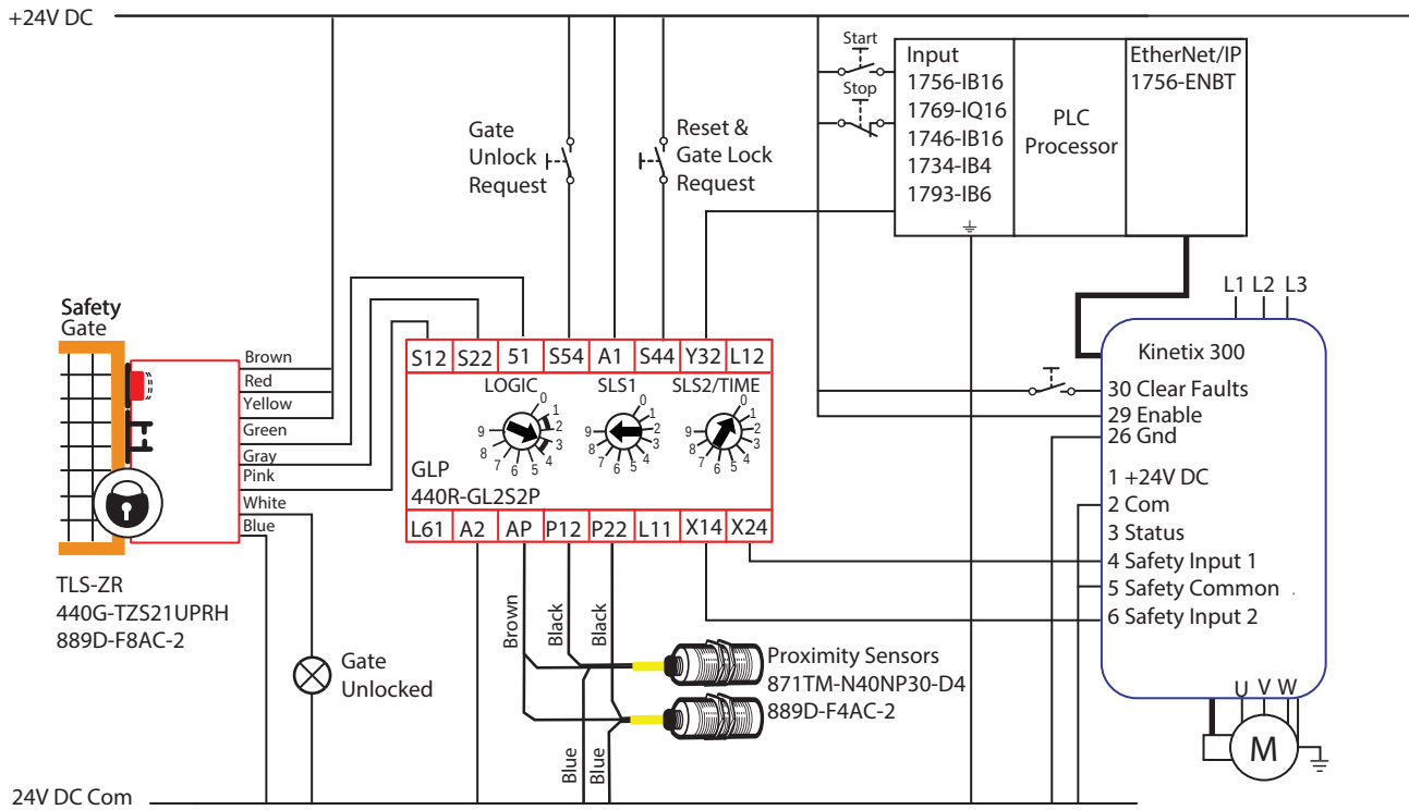
Figure 40 - Safely-limited Speed with Guard Locking Interlock and Proximity Sensors
