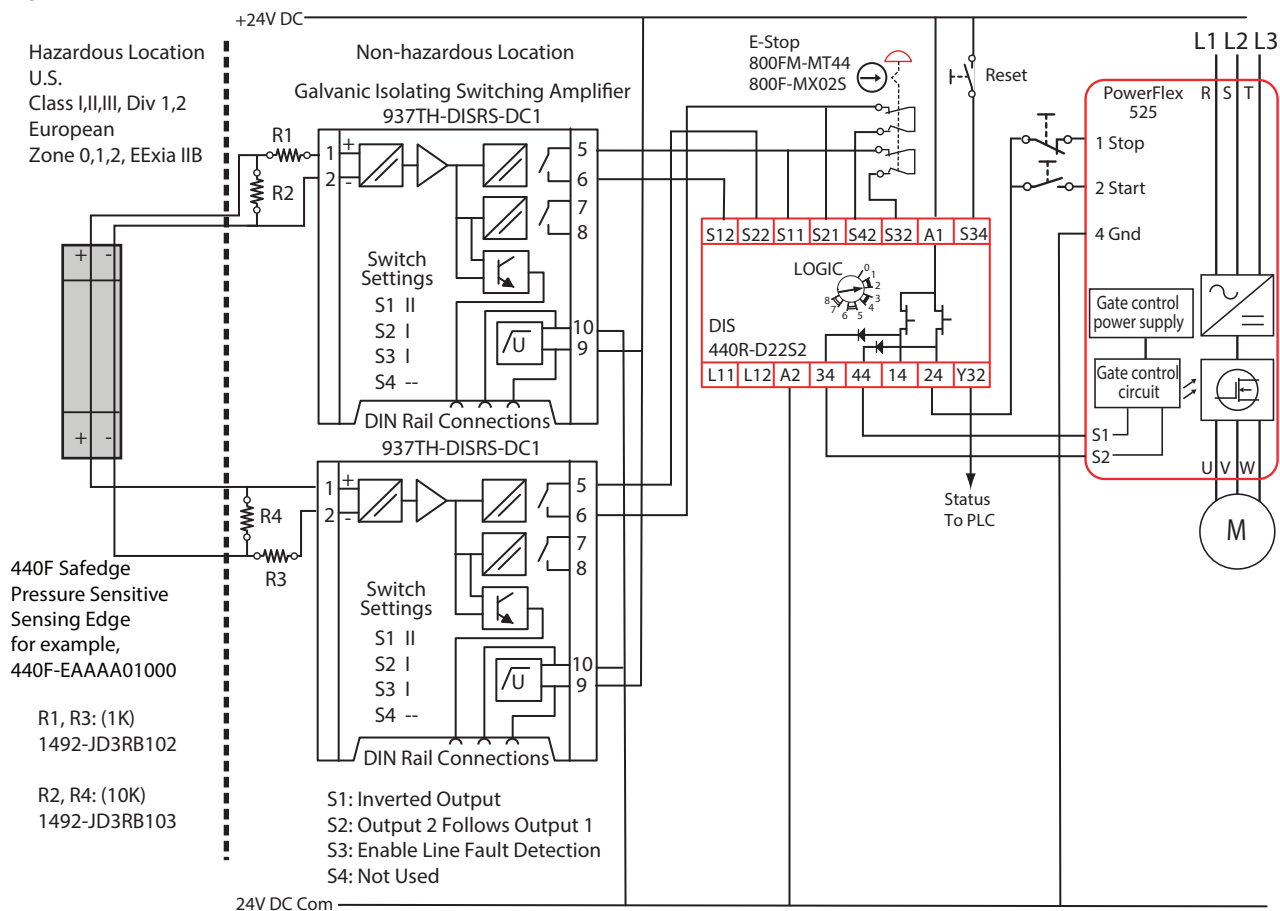
Figure 31 - Hazardous Location
