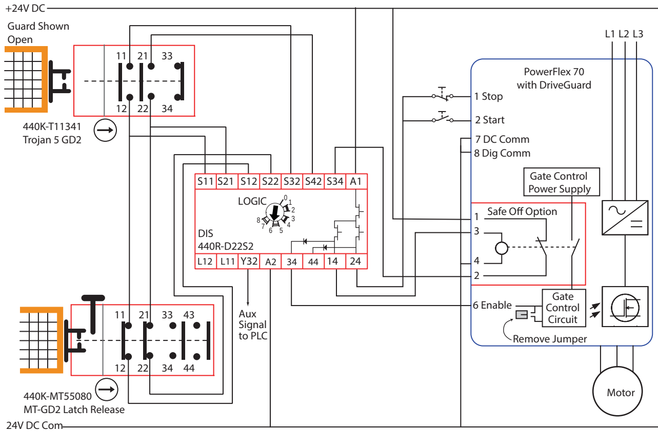
Figure 32 - PowerFlex Drive - Multiple Gate Access
