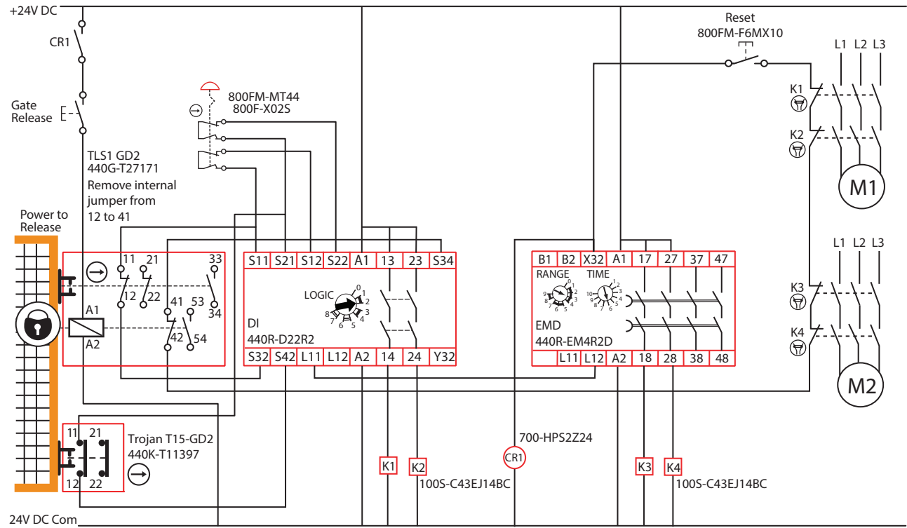
Figure 22 - Guard Locking with DI/EMD Safety Relays
