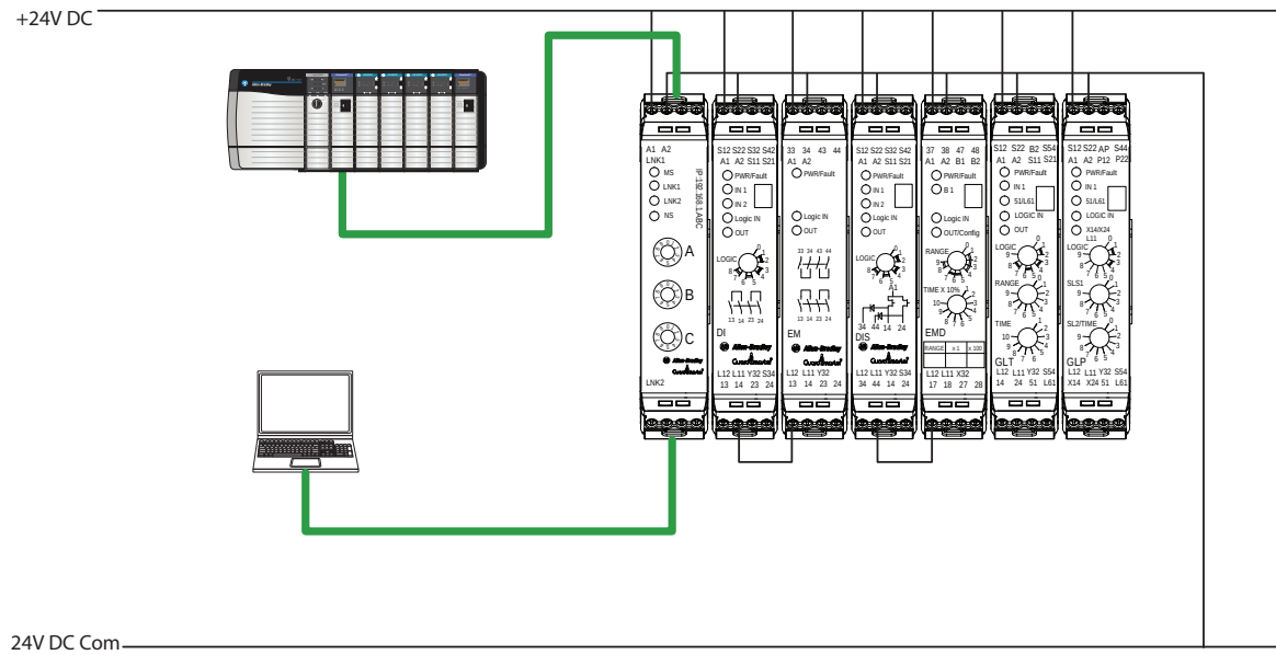
Figure 56 - EtherNet/IP to Logix Controllers
