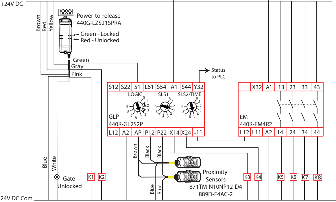
Figure 42 - Stop Motion with Guard Locking and E-stop
