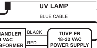
ER (low-voltage) models wiring
