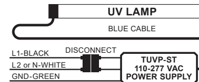
ST (line-voltage) wiring
