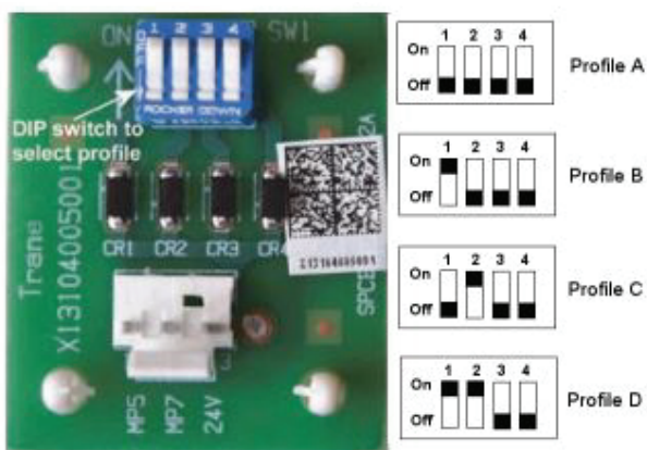
Figure 64. Units with UC400 controls and ECM motors -DIP switch settings
