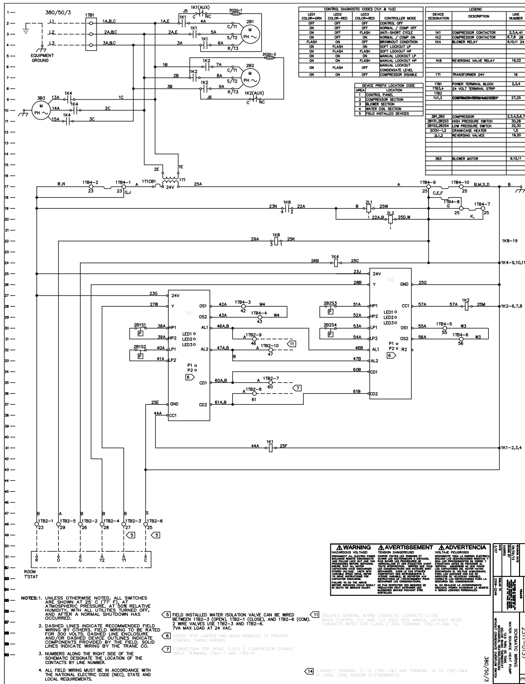
Figure 83. GEH_V (6 to 25 tons) - deluxe 380V - 420V - 50 Hz - 3 ph
