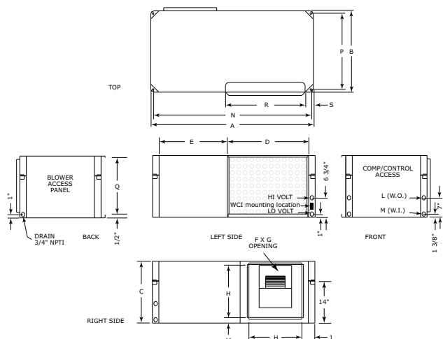
Figure 8. Left return/right supply (GEHE)
