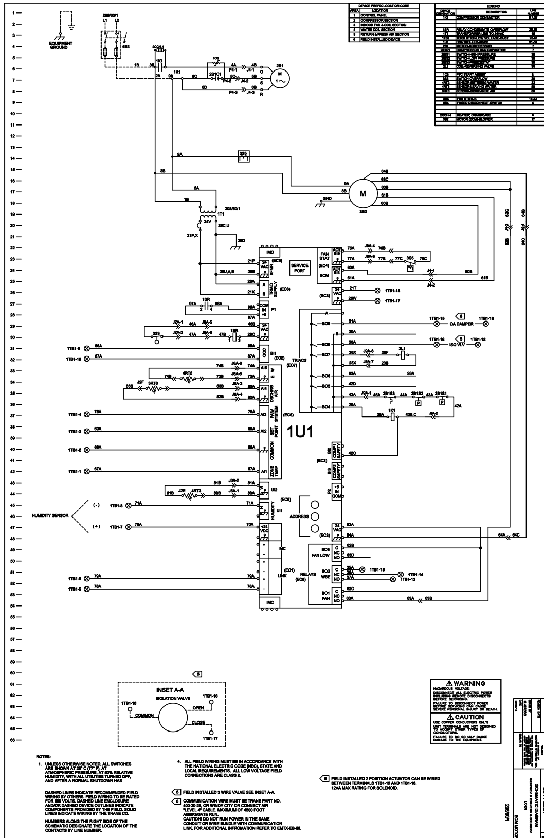
Figure 86. GEHE (0.5 to 1.5 tons) - UC400
