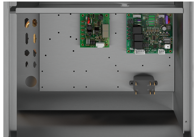
Figure 62. ECM control box
