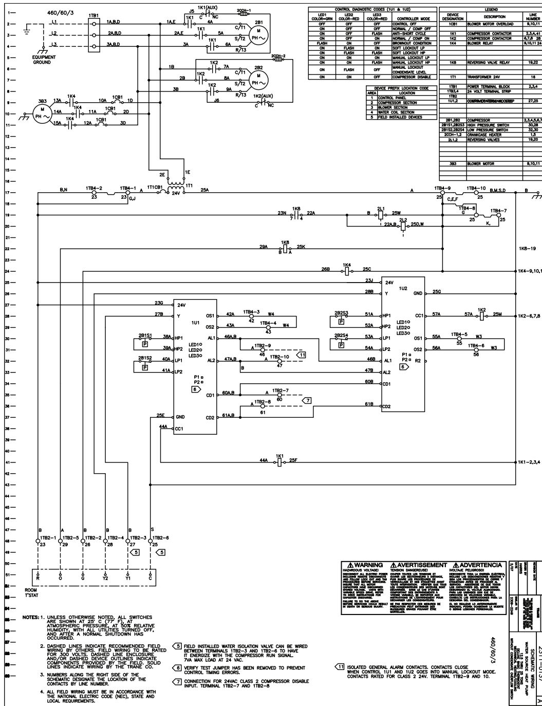
Figure 84. GEH_V (6 to 25 tons) - deluxe 24V - 460V - 60 Hz - 3 ph
