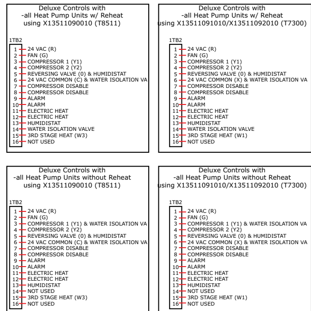
Figure 55. Low-voltage connection (GEH/V 6 to 25 ton)
