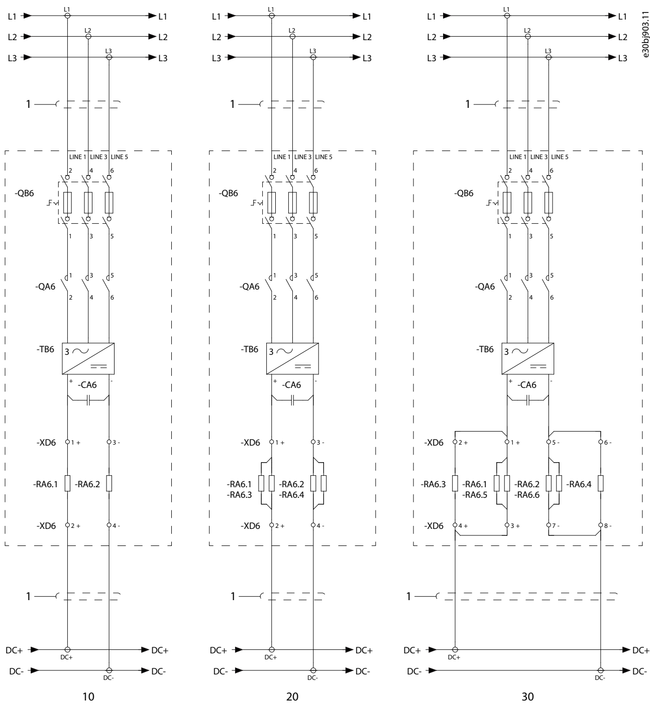
Illustration 7: Main Circuits of the Pre-charging Units
