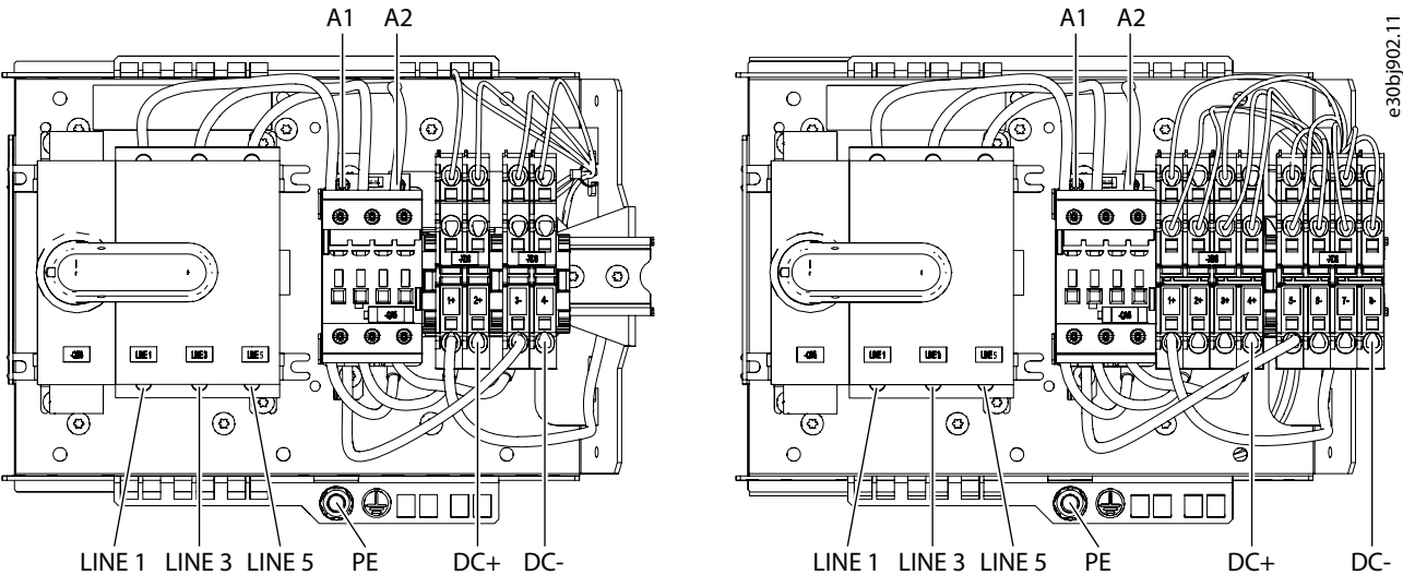
Illustration 6: Terminals of the Pre-charging Unit
