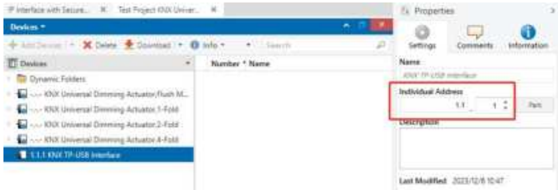
Fig.4.2 ETS project properties window--setting the desired individual address
