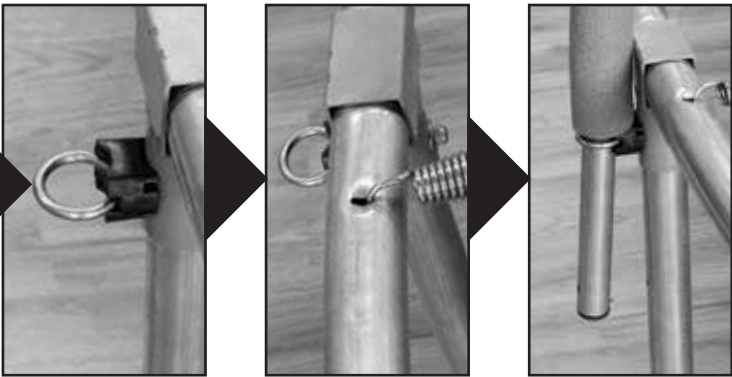
5 Align the opening on the pole cap with the spring-loaded button on the top of the Upper Poles. Then, slide the Pole Caps (Q) over all 8 Upper Pole assemblies until the buttons click into place.
