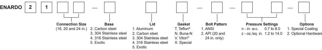
Figure 2. Enardo 2100 Series Model Number Identification
