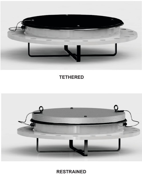
Figure 3. Enardo 2100 Series Product Configurations
