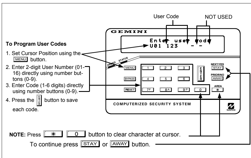
Programming User Codes with GEM-K1CA Keypad
