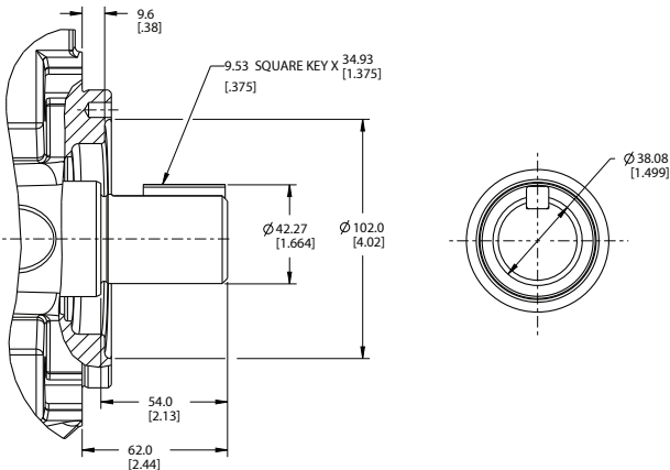
10 - SAE J744-38-1 SAE C-C STRAIGHT KEYED
