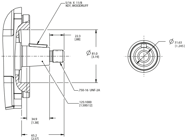
24 - 24 - 31.8 [1.25] DIA TAPERED KEYED SHAFT .750-16 UNF-2A EXTERNAL THREAD KEY INCLUDED
