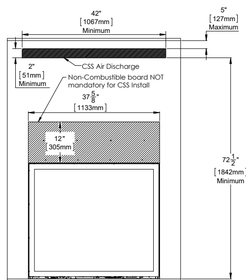
Figure 1: Framing Option 1
