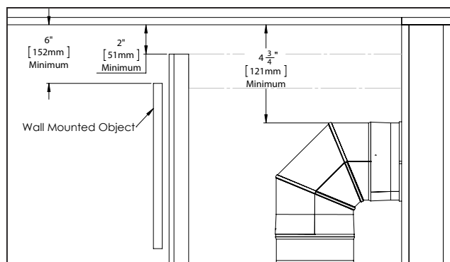
Figure 2: Open Chase
