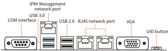
Figure 1-2 Rear I/O panel
