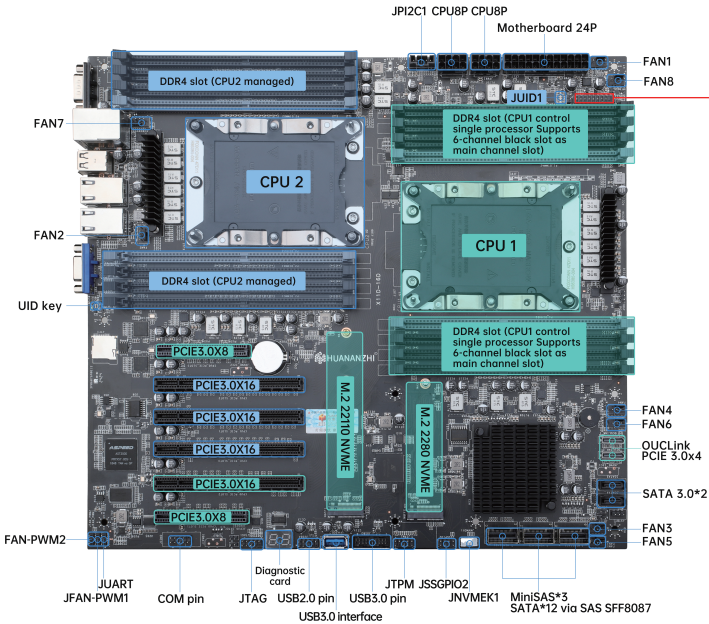
Figure 1-1 X11D-16D dual mainboard diagram
