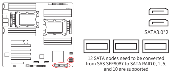
Figure 2-6 SATA ports
