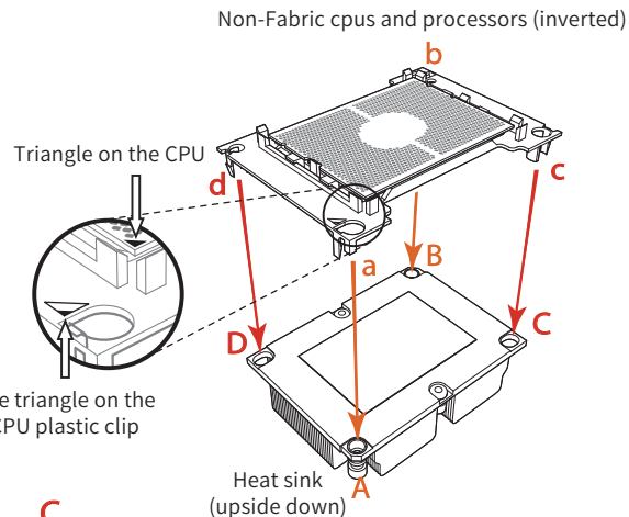
Figure 2-10 Installing a CPU
