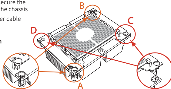
Figure 2-10 Installing a CPU
