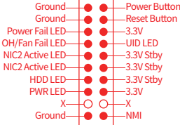
Figure 1-1 X11D-16D dual mainboard diagram
