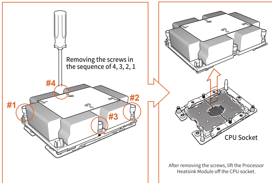
Figure 2-13 Removing a CPU
