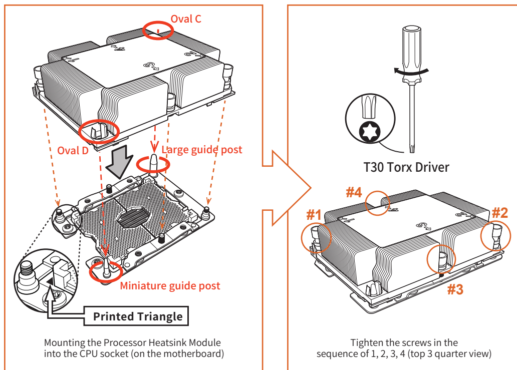
Figure 2-12 Installing a CPU
