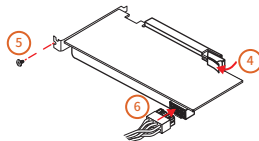
Figure 2-9 Video card installation
