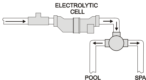
Inverted Installation
