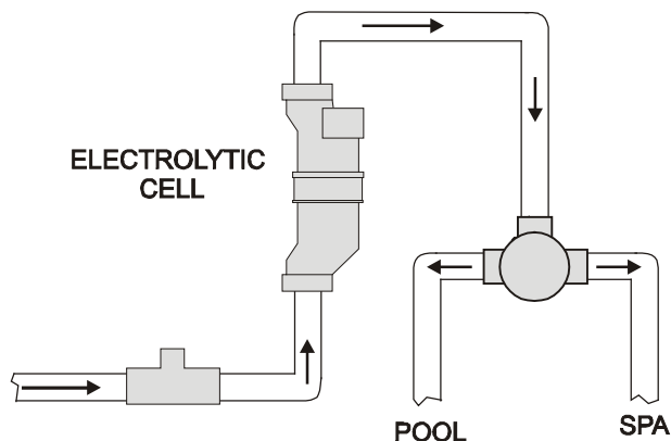
Vertical Installation
