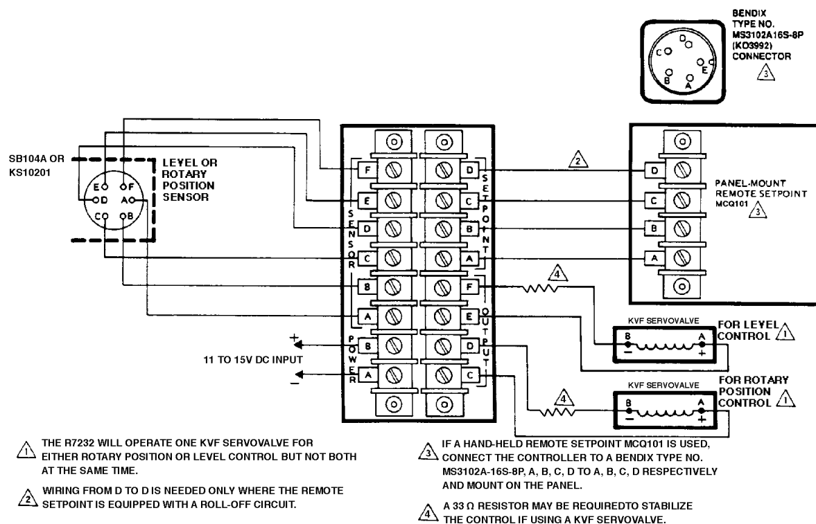
Typical System Wiring to an R7232A With Terminal Strips.
