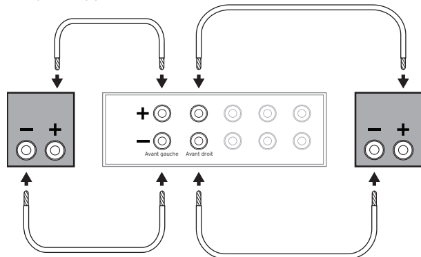
FIGURE 3 BRANCHEMENTS STANDARD
