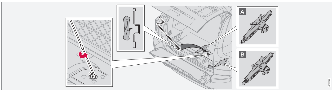
Jack location
