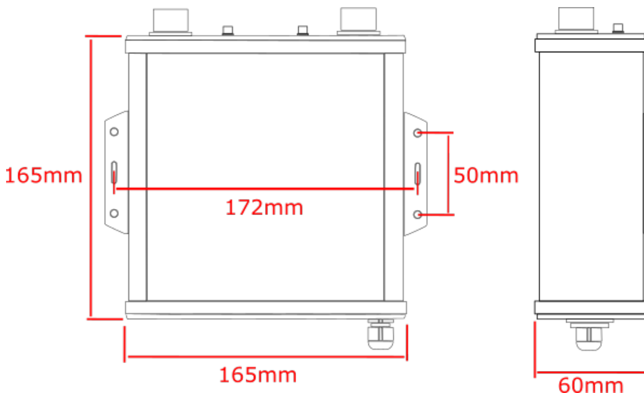
Figure 1 - Dimensions
