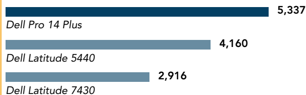
Figure 8: Procyon Photo Editing Benchmark measures CPU performance. This content creation benchmark uses Adobe® Photoshop® and Lightroom® Classic applications to mimic a “typical photo editing workflow that includes batch processing and image retouching.” 18 Source: PT.
