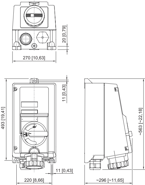
Prise murale
