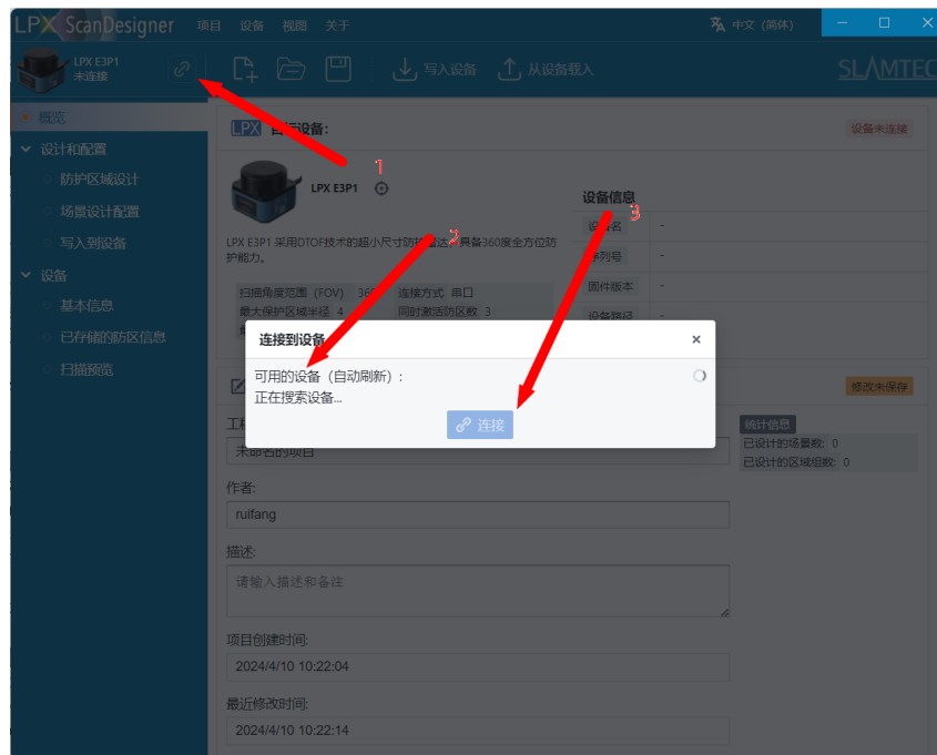
Figure 4.1: Devise connecting GUI
