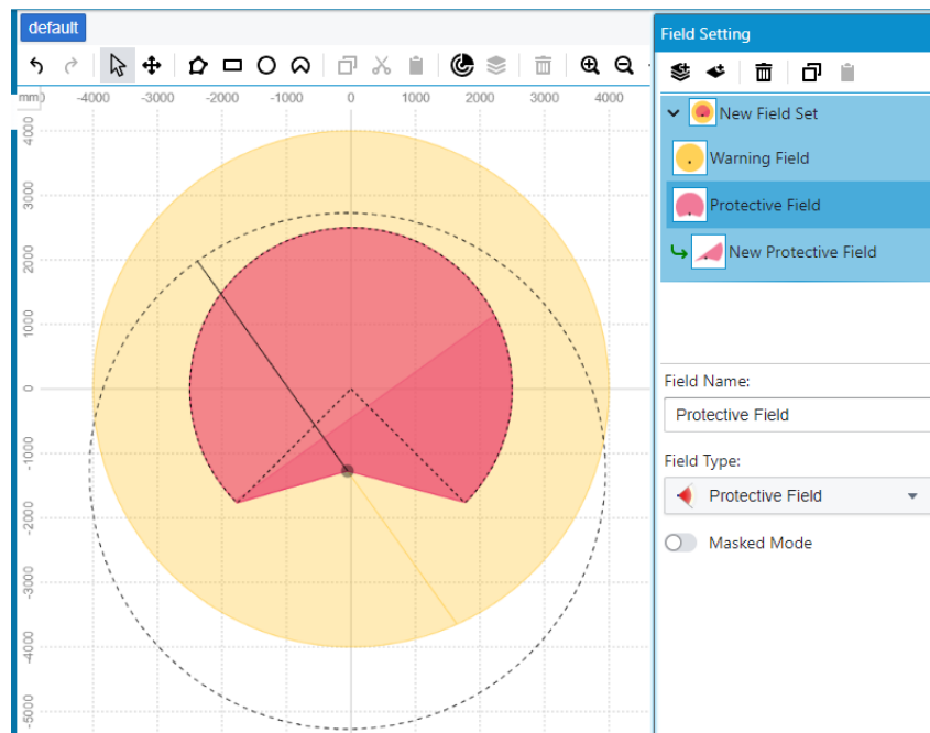
Figure 5.12: Adjust lidar position
