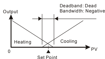
Figure 6: PID Control
