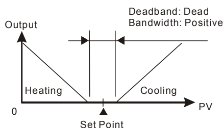
Figure 5: PID control
