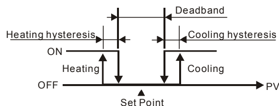
Figure 4: ON/OFF Control
