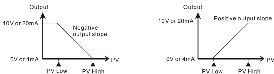
Figure 7: Proportional Output
