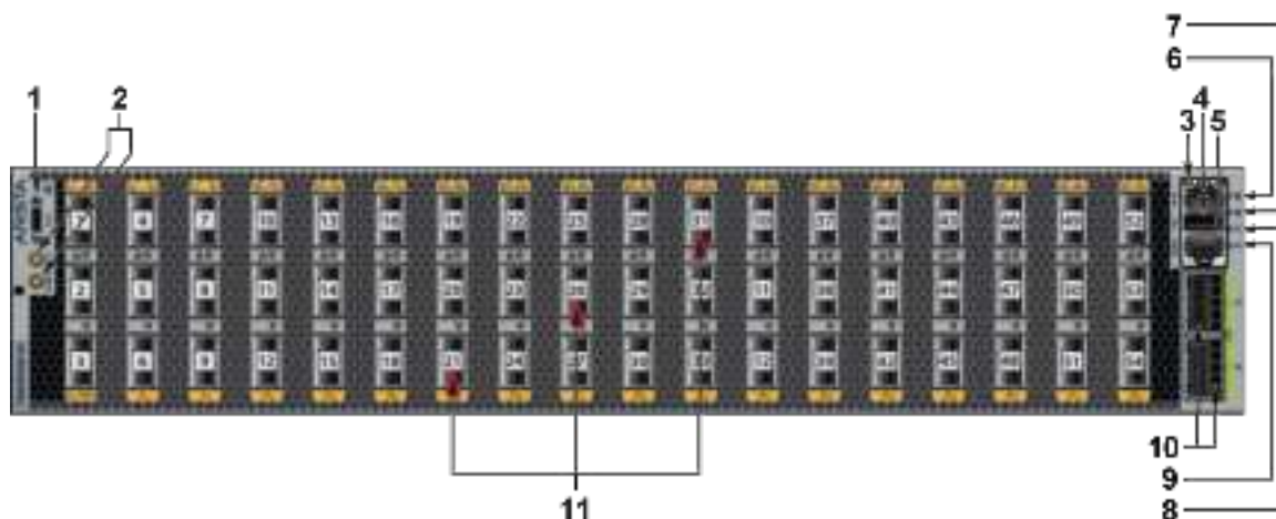
Figure 48: DCS-7280DR3A-54, DCS-7280DR3AK-54 and DCS-7280DR3AM-54
