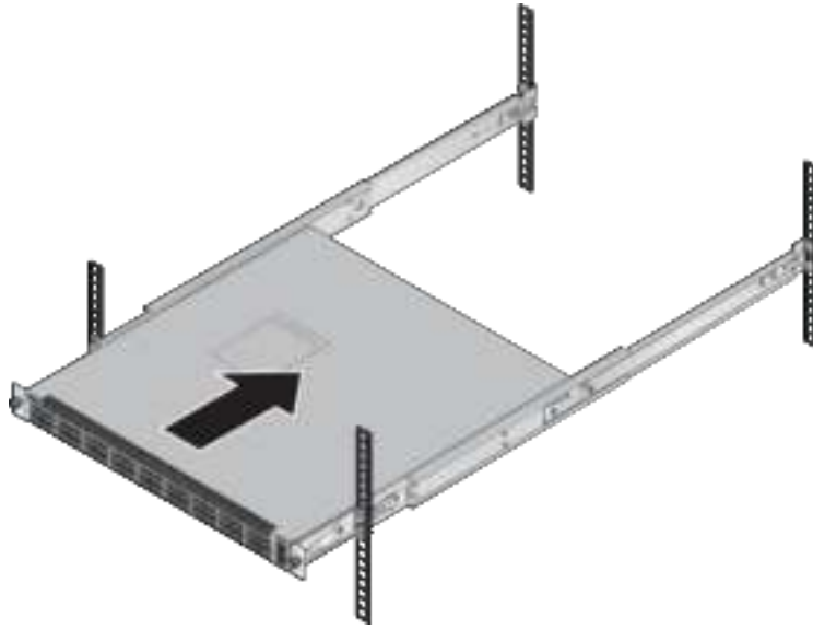
Figure 14: Inserting the Switch onto the Rails
