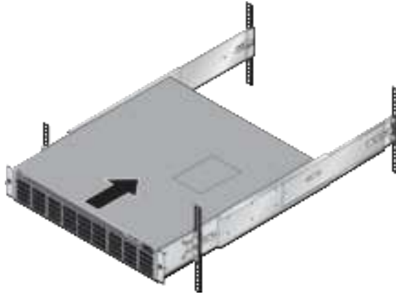
Figure 20: Inserting the Switch onto the Rails
