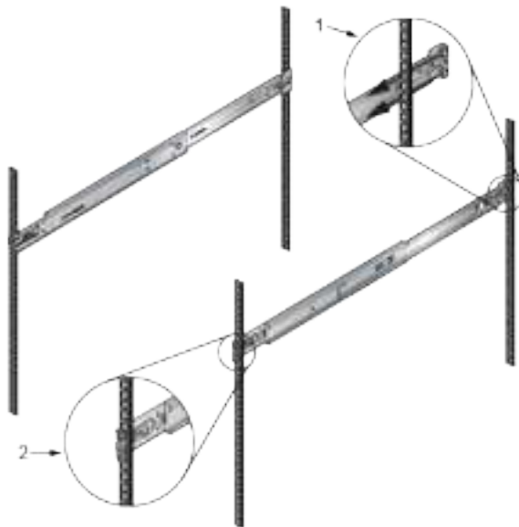
Figure 13: Attaching the Rails
