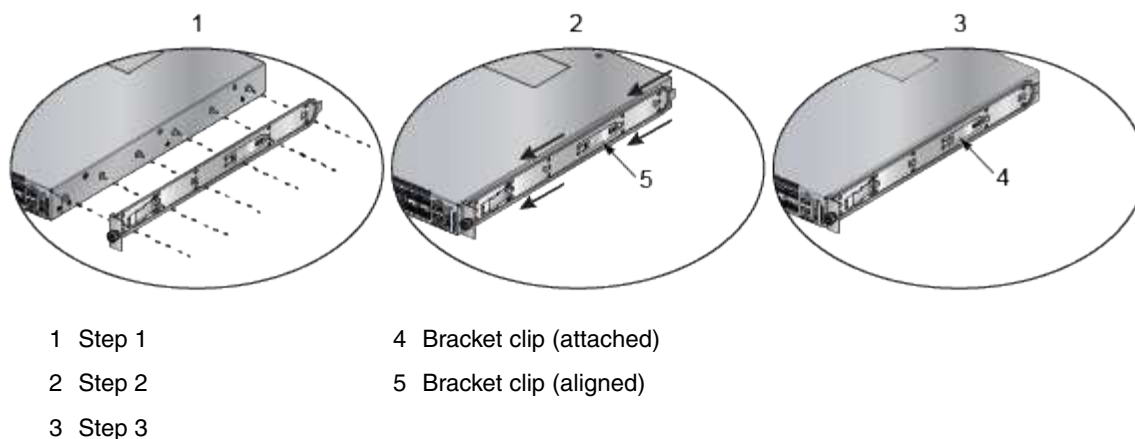
Figure 11: Attaching the Four-Post Mounting Brackets to the Switch Chassis
