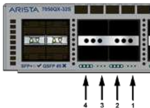
Figure 33: Port LEDs
