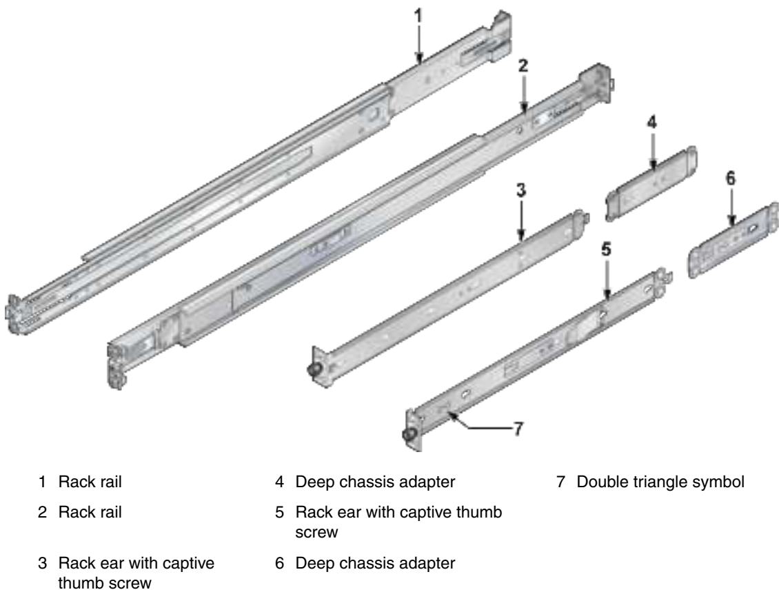
Figure 39: Four-Post Rack Mounting Brackets with Roller Extensions
