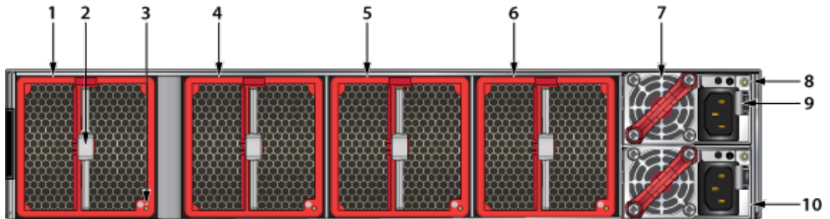
Figure 53: Rear Panel with Separation Between Fans 1 and 2 (no ground)
