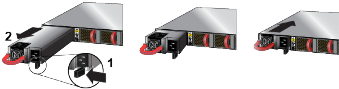
Figure 54: Removing and Installing Power Supply
