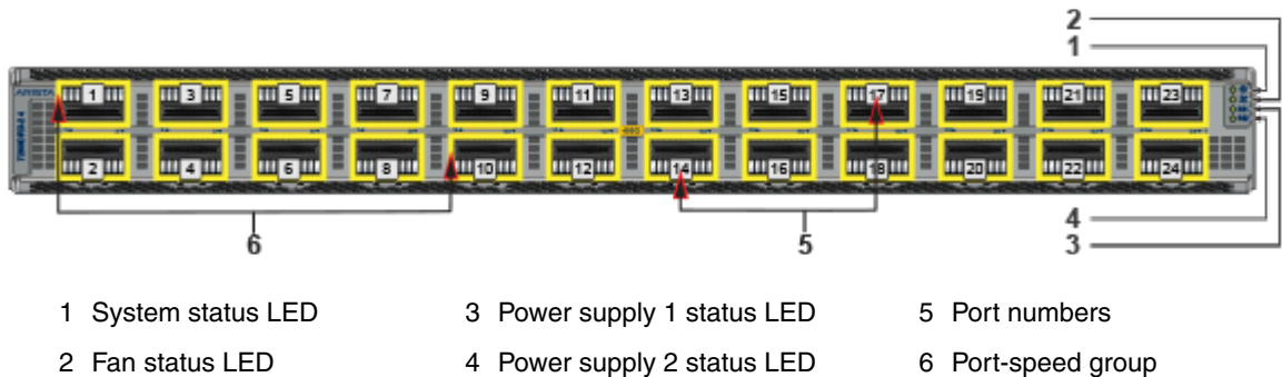
Figure 42: DCS-7280CR3-32P4, DCS-7280CR3K-32P4 and DCS-7280CR3K-32P4A
