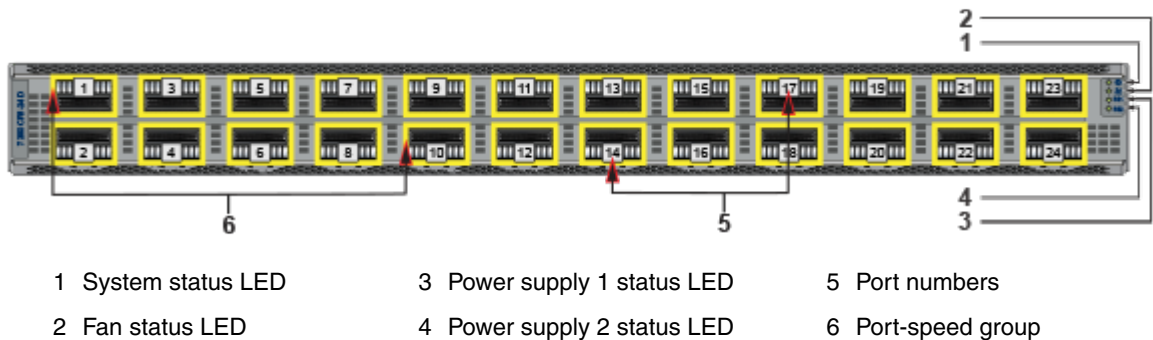
Figure 41: DCS-7280DR3-24 and DCS-7280DR3K-24
