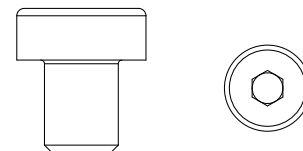
Screw M4 x 5 DIN7984 (8 pcs)
