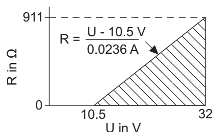
Fig. 26: Maximum load resistance as a function of an external power supply voltage
