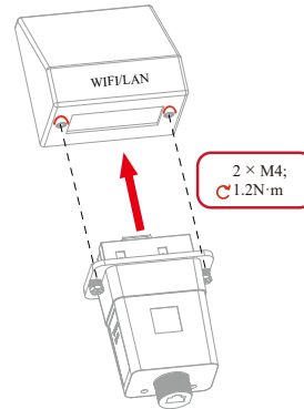
2. Install the module.
