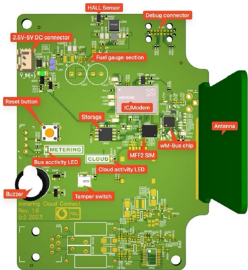
components on the PCBA
