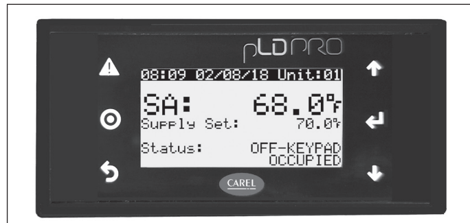
Figure 2.3 - Unit Mounted pLDPRO Interface
