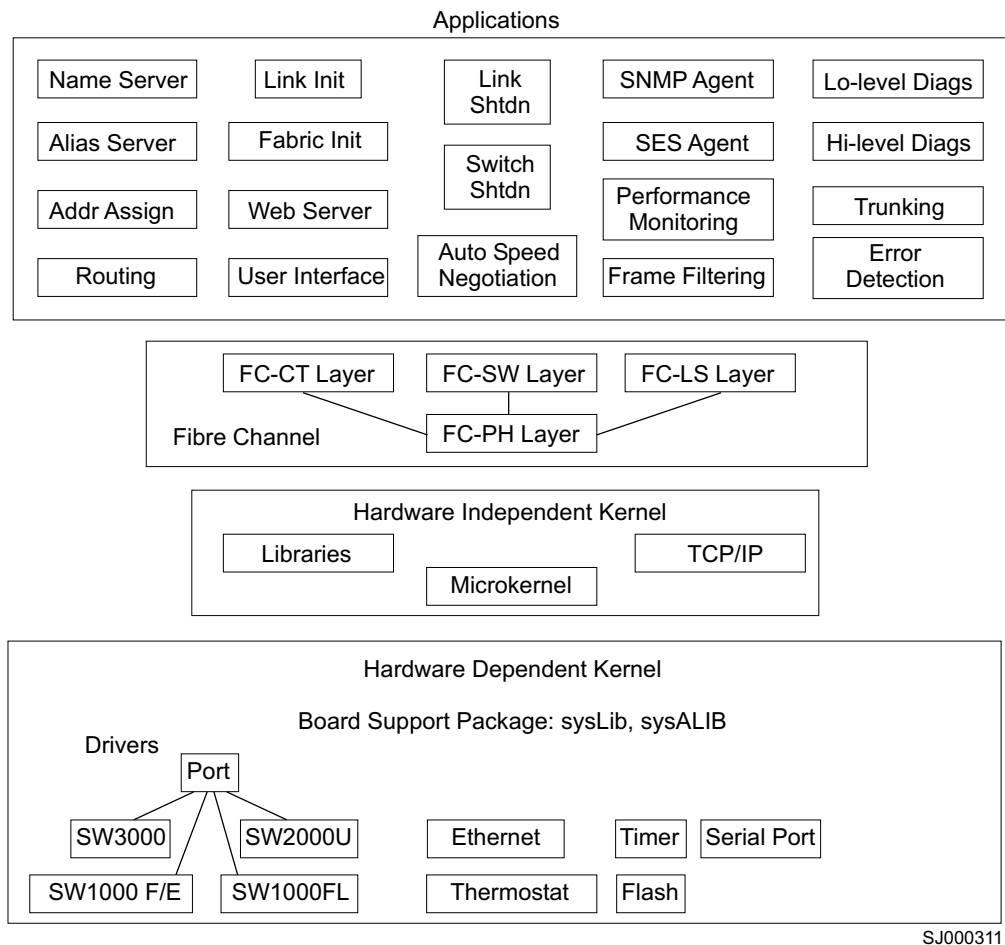
Figure 6. 3534 Model F08 firmware components
