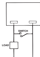
FIG. 2 POST PURGE
