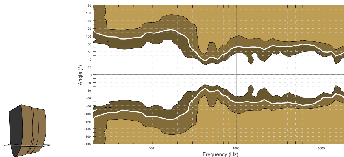
Dispersion angle diagram of one L2D at 140^\circ with a cardioid pattern, using lines of equal sound pressure at -3 dB, -6 dB, -12 dB.
