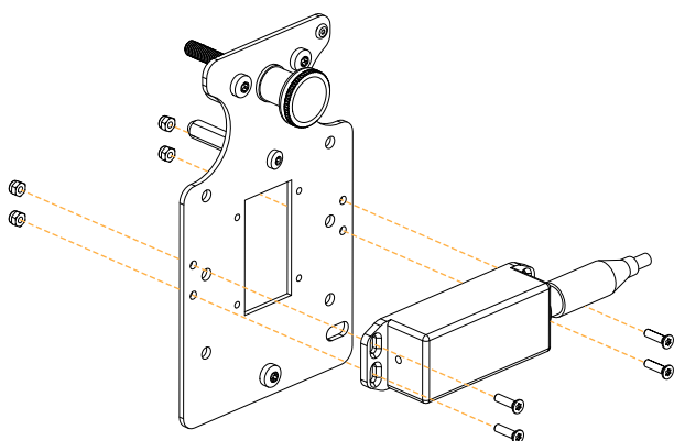
Vertical mount
