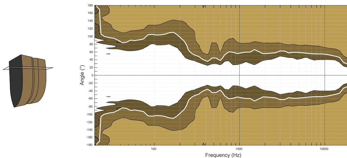
Dispersion angle diagram of one L2D with 110^\circ fins settings and a cardioid pattern, using lines of equal sound pressure at -3 dB, -6 dB, -12 dB.
