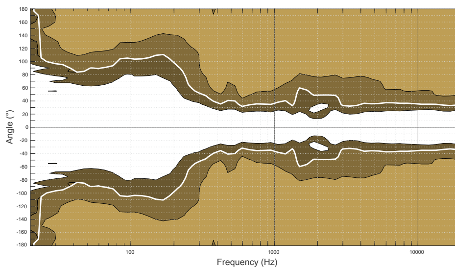
Dispersion angle diagram of one L2 with 70^\circ fins settings and a cardioid pattern, using lines of equal sound pressure at -3 dB, -6 dB, -12 dB.
