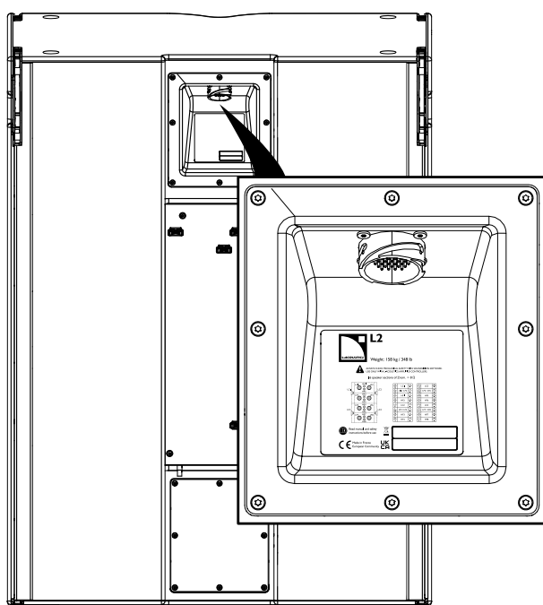
L2 1 x 37-point male connector (32 points used)
