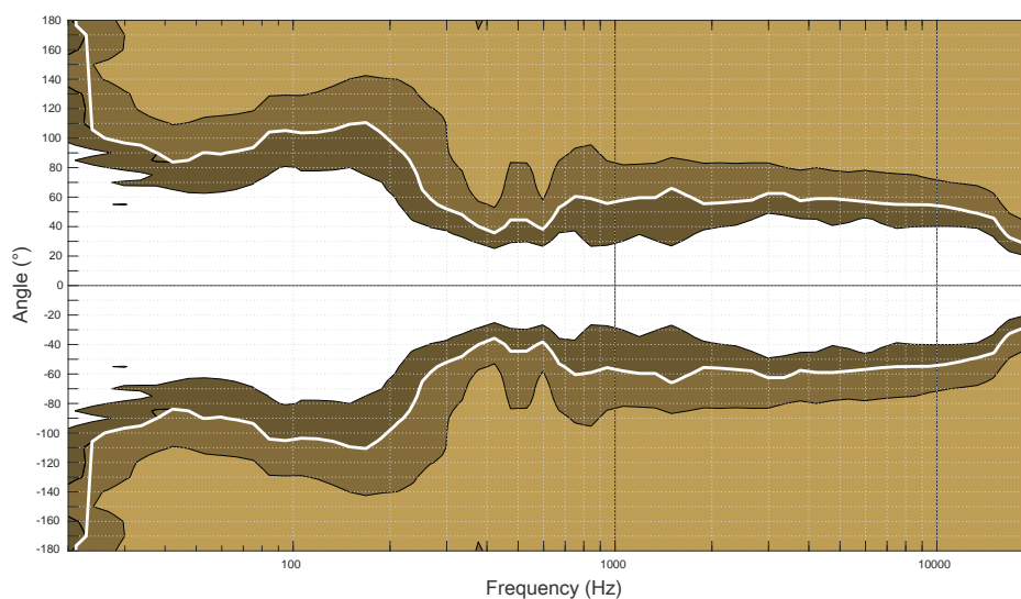
Dispersion angle diagram of one L2 with 110^\circ fins settings and a cardioid pattern, using lines of equal sound pressure at -3 dB, -6 dB, -12 dB.
