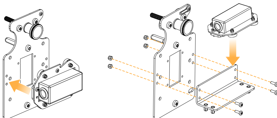
Vertical mount
