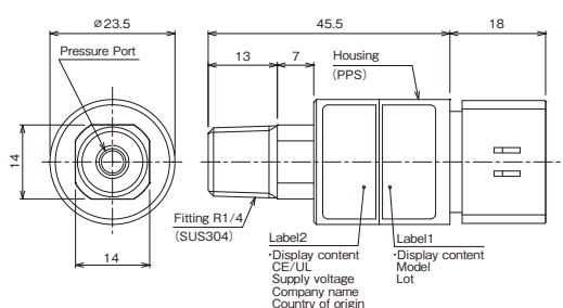
(2) PA-750 Configurations of joint R2 (R1/4)
