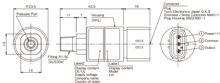
(1) PA-750 Configurations of joint R1 (R1/8)
