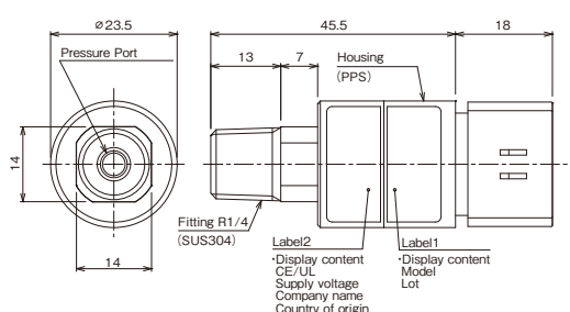
(5) PA-758 Configurations of joint R2 (R1/4)
