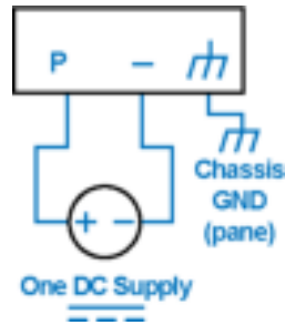
Figure 12: Power Wiring Diagram
