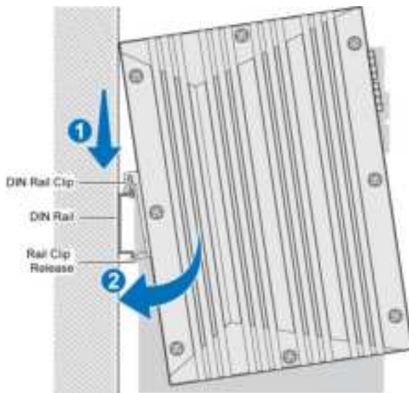
Figure 8: Installing the DIN-Rail Kit
