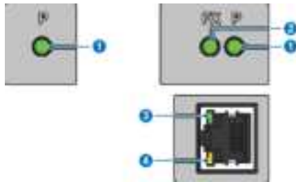
Figure 3: Front Panel LEDs for JetNet 2205 Series
