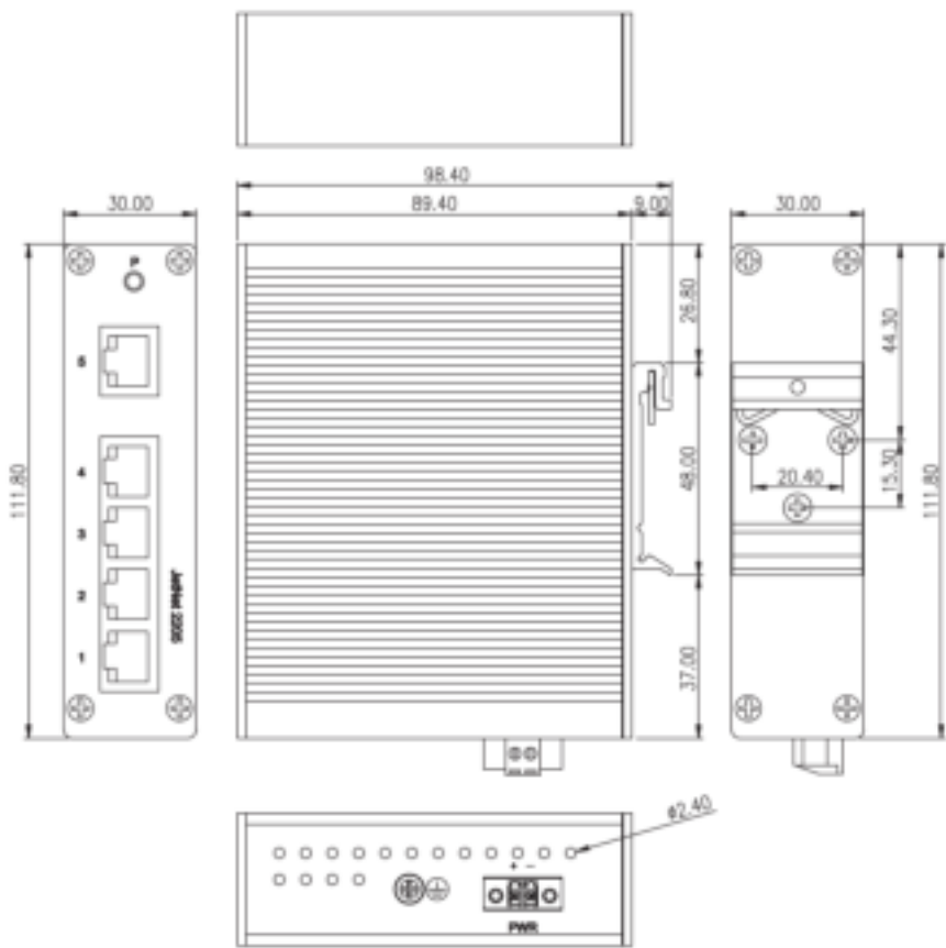
Figure 6: Dimensions of 5-Port JetNet 2205
