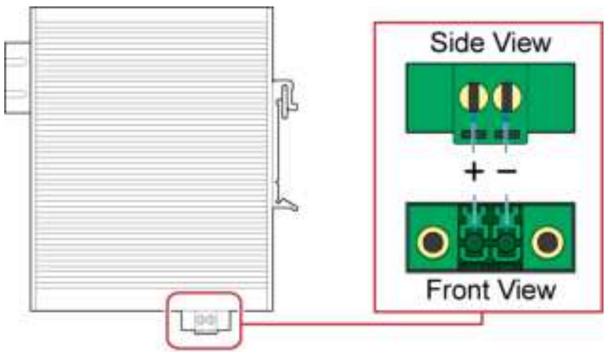
Figure 14: Terminal Block Side and Front Views
