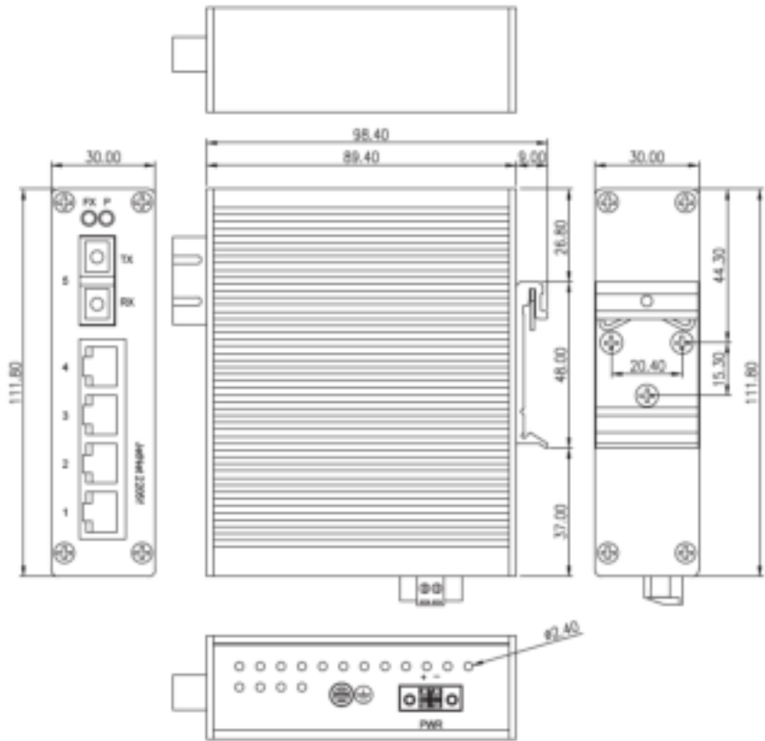
Figure 7: Dimensions of 5-Port JetNet 2205f
