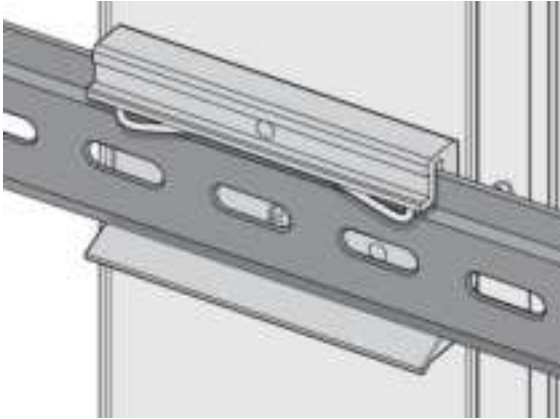
Figure 9: Example of an Installed DIN Rail Kit
