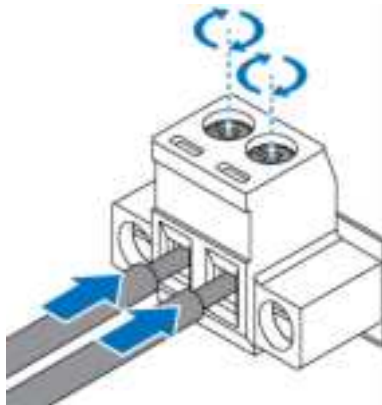
Figure 15: Installing Power Cabling in a Terminal Block
