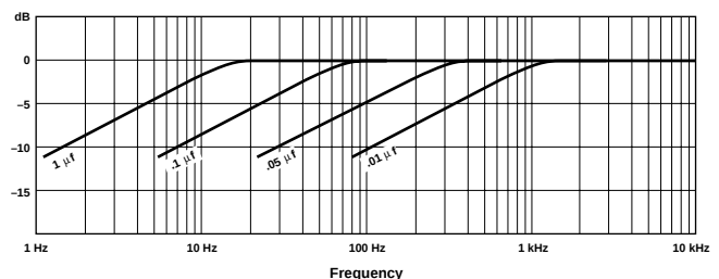
Fig. 3.10 Subsonic Filter Capacitor Values
