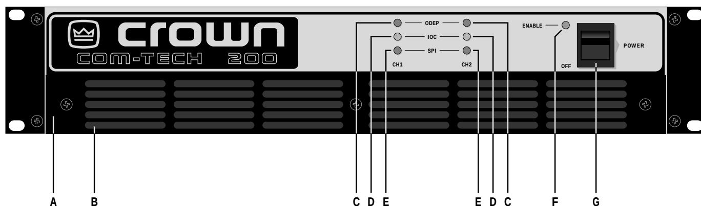
Fig. 2.1 Front Facilities
