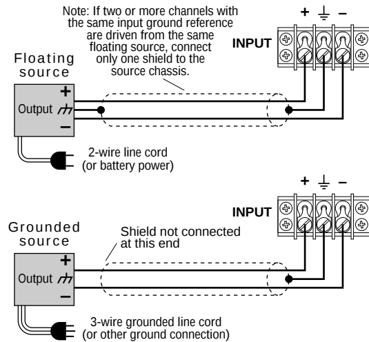
Fig. 3.9 Balanced Input Wiring
