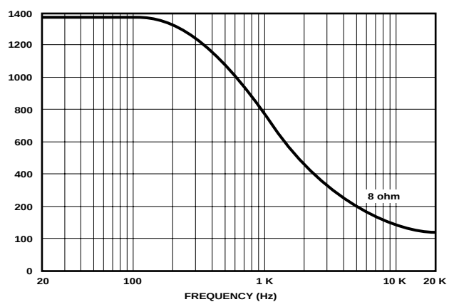
Fig. 6.10 Typical Damping Factor
