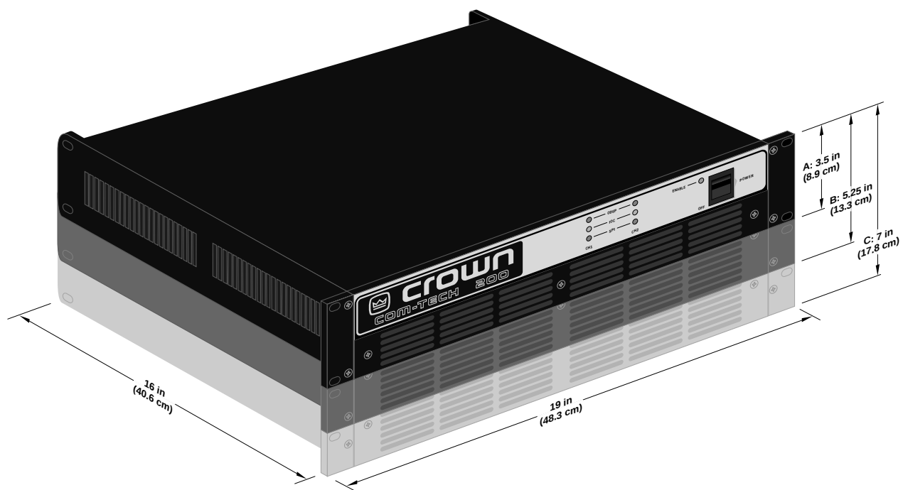
Fig. 3.1 Mounting Dimensions
