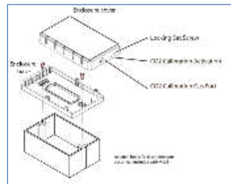
Figure 3: Attaching to single gang box.
