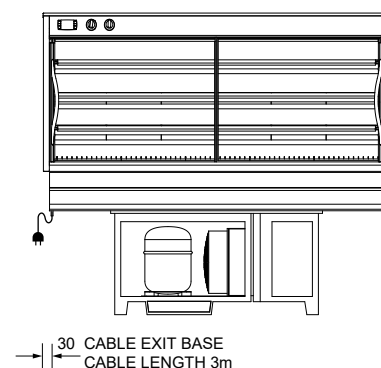
REAR ELEVATION
