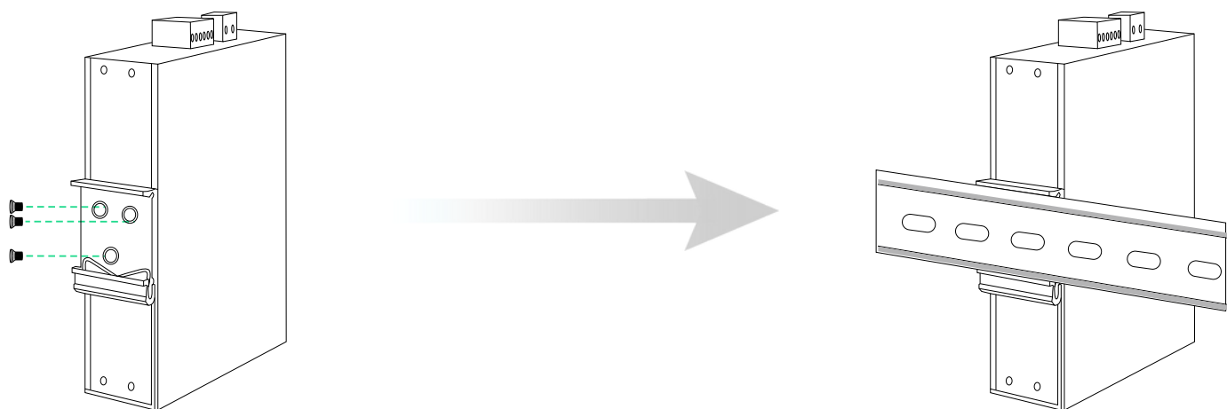
DIN-Rail Mounting
