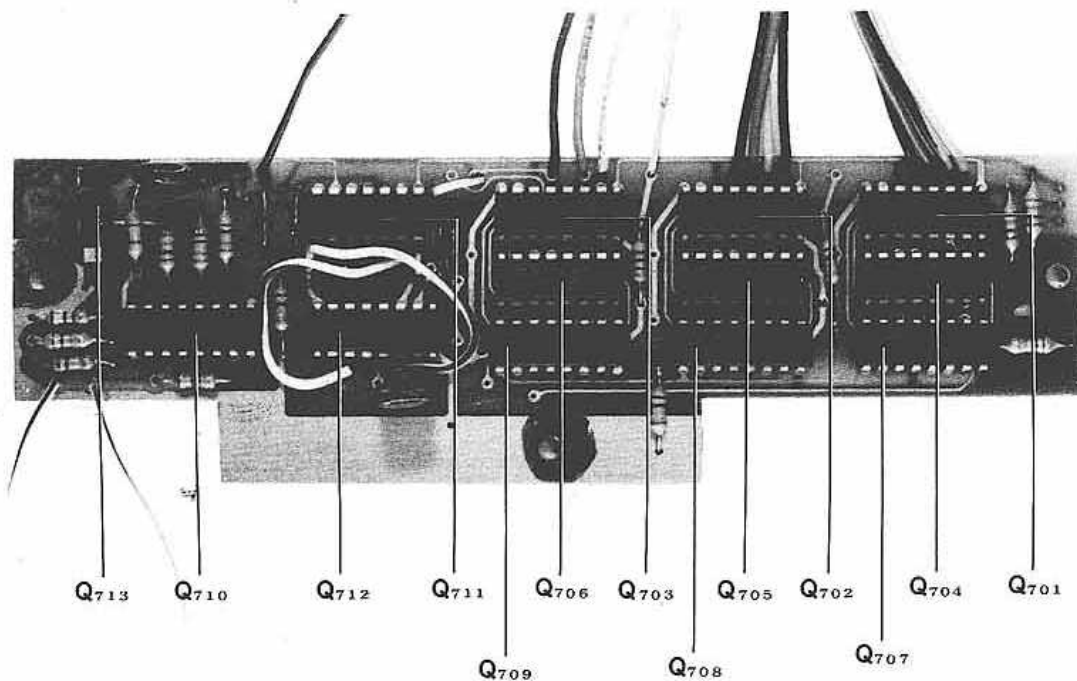
PLL CONTROL UNIT
