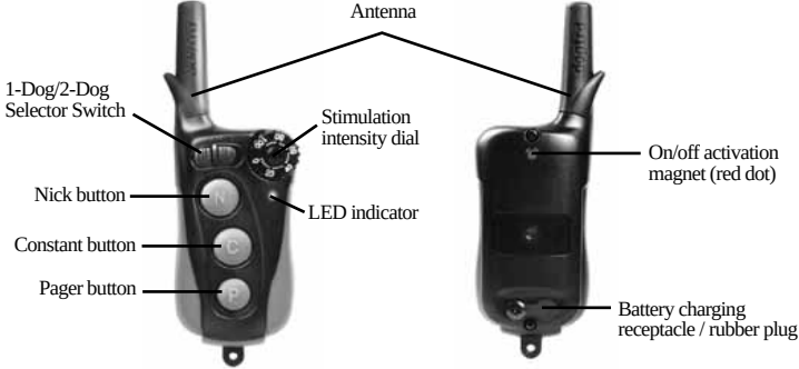
Handheld Transmitter
