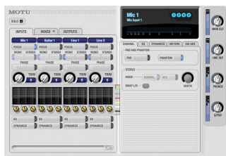
Figure 6-1: CueMix FX.
