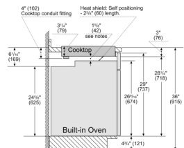
30" Built-in oven - under induction cooktop
