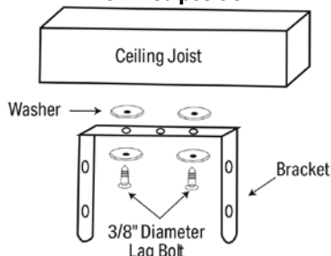
FIGURE 4b: Double-screw mounting, for fixed position
