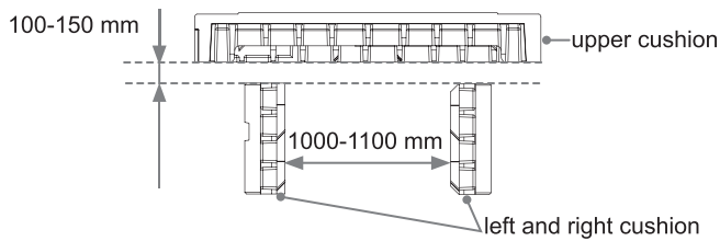
Figure 1. Top View
