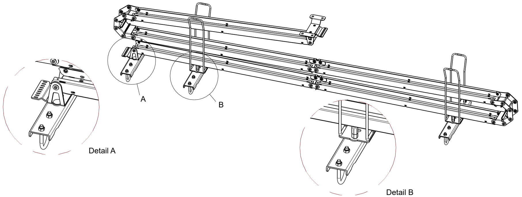
Snake extension 30 truss
